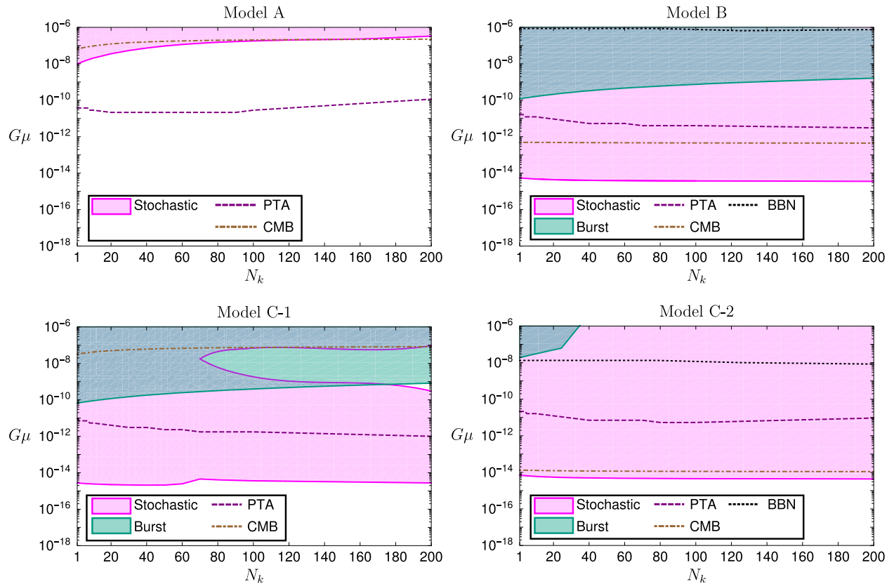
FIG. 3. Exclusion regions at 95% C.L. on the cosmic string parameter space (N_k, G\mu) derived from the stochastic search (pink) and the burst search (turquoise). Four models are considered to describe the distribution of cosmic string loops: model A (top left), model B (top right), model C-1 (bottom left), and model C-2 (bottom right). Note that the stochastic result combines the data of O1, O2, and O3, while the burst search only includes O3 data. We also report limits from other experiments: pulsar timing arrays (PTA) [33,34], cosmic microwave background (CMB) [31], and Big Bang nucleosynthesis [32]. The notch in the SGWB constraint for model C-1 is explained in the Supplemental Material [42].
