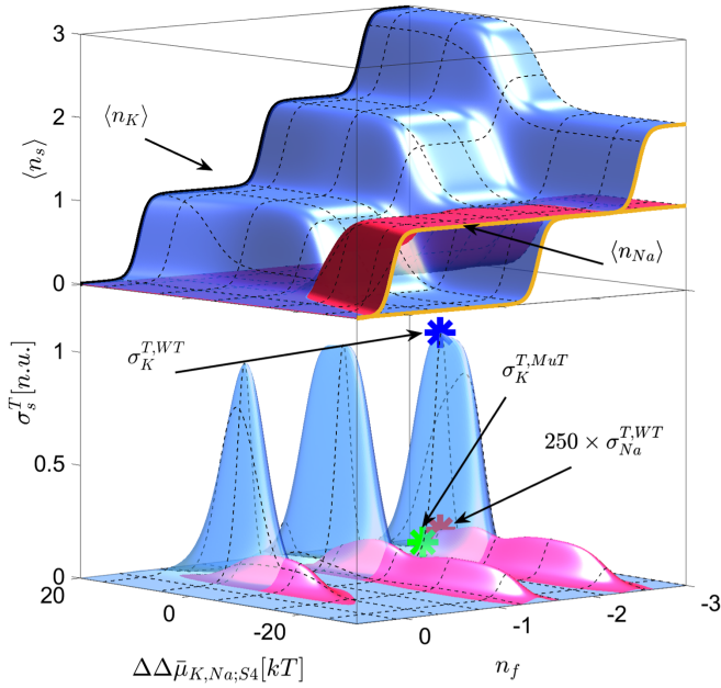
FIG. 3. K^+ (blue) and Na^+ (red) occupancy (top) and conductivity (bottom) vs n_f and \Delta\bar{\mu}_{K,Na;S4} in symmetrical 0.2M mixed species bulk solutions. Conductivity and occupancy form a set of resonant peaks and steps, respectively. Peaks maximize under the condition of barrierless knockon, it being the favored species and minimal difference in site affinity. Using identical parameters to Fig. 2, we indicate the WT K^+ (blue) and Na^+ (red) and MuT K^+ (green) conductivities via colored stars. Selectivity appears via the shift in both occupancy and conductivity from K^+ (blue) to Na^+ (red) surfaces, and the conductivity ratio yields \sigma_K^{T,WT}/\sigma_{Na}^{T,WT} \sim 2 \times 10^3 .
