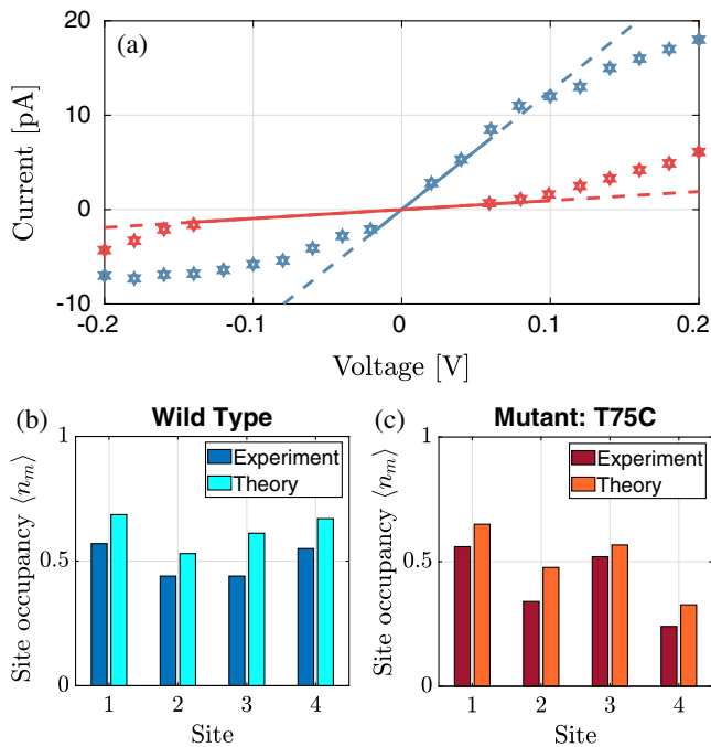
FIG. 4. Comparison of theoretical current (a) (lines), and site occupancy (b) and (c) to experimental data [13] denoted by stars in (a) and as labeled in (b) and (c). Theory and data are shown for the WT in blues and for the mutant (MuT) in reds. By comparison we find \Delta\bar{\mu}_{K,1-3} \sim 6.2, 5.7, 6kT , \Delta\bar{\mu}_{K,4}^{WT} \sim 6.2kT and \Delta\bar{\mu}_{K,4}^{MuT} \sim 5.2kT , a diffusivity in the channel of 2.3 \times 10^{-10} \text{ m}^2 \text{ s}^{-1} . The charge of the mutant was estimated as n_f \sim -2.32 .
