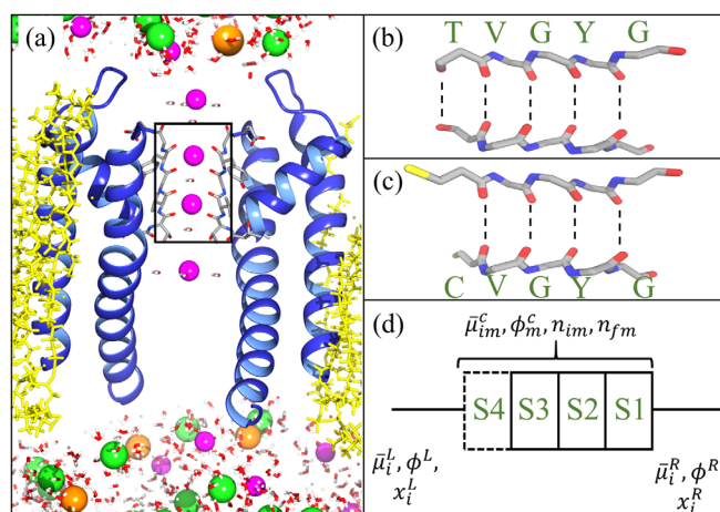
FIG. 1. Structure of open KcsA (5vk6.pdb) [10] visualized using Chimera [11]. (a) Two chains (blue ribbons) spanning a lipid membrane (yellow strands) between two aqueous ionic solutions. The SF is located within the box, and K + (purple), Na + (orange), and Cl - (green) ions alongside water molecules are included. (b) Structure of the SF for wild type KcsA and (c) the T75C mutant, with indicated amino acids at binding sites. (d) Lattice model used to define the system.
