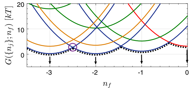
FIG. 2. Free energy vs n_f with KCl and NaCl solutions at 0.2M . Only the most favored states are included. Colors red, blue, green, orange, and black dashed lines denote empty, pure \text{K}^+ or \text{Na}^+ , mixed i.e. \text{K}^+ and \text{Na}^+ , and the ground states, respectively. The purple circle shows when the pore is equally favorable to hold 2 or 3 \text{K}^+ ions. \Delta\bar{\mu}_{\text{K},1-4} in are \sim 6.2, 5.7, 6, 6.2kT while \Delta\bar{\mu}_{\text{Na},1-4} are \sim 2.2, -2.6, -1.6, 0.1kT .
