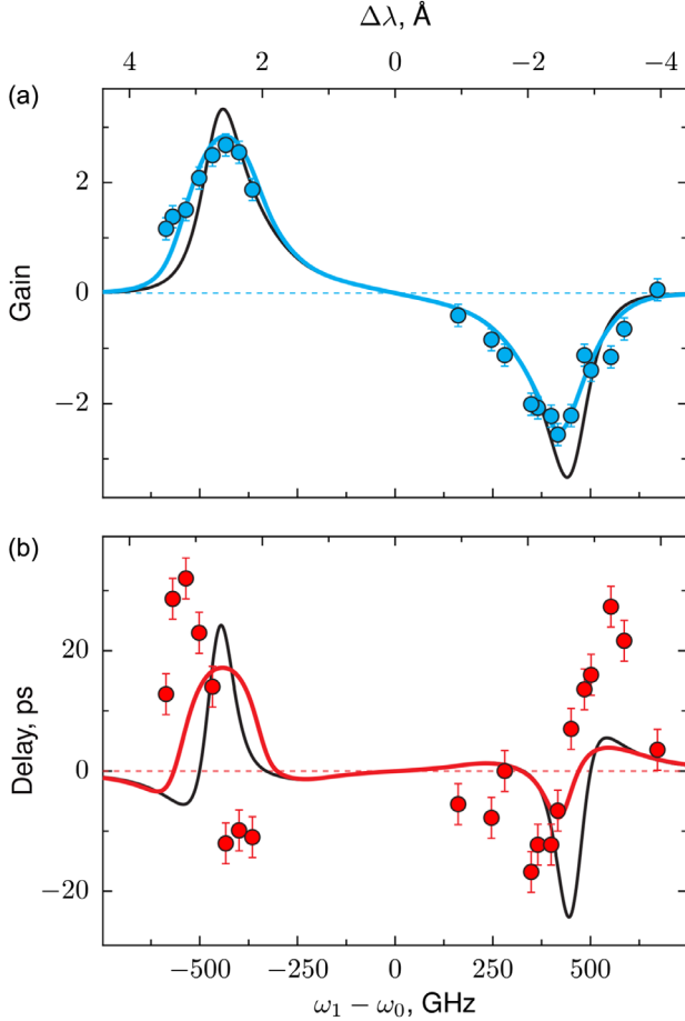
FIG. 4. Experimental measurement of slow and fast light compared to theory. (a) The measured gain (blue circles) compared to linear theory calculations with (blue) and without (black) compensation for the finite f number of the pump ( f/6.7 ) and probe ( f/10 ) for both the slow light ( \Delta\lambda < 0 ) and fast light ( \Delta\lambda > 0 ) sides. (b) The measured pulse delay compared to linear theory calculations with (red) and without (black) compensation for the finite f number. For both plots, the theory curves are calculated for n_e = 1.25 \times 10^{19} \text{ cm}^{-3} , T_e = 256 \text{ eV} , T_i = 45 \text{ eV} , and I_0 = 3.25 \times 10^{13} \text{ W/cm}^2 .
