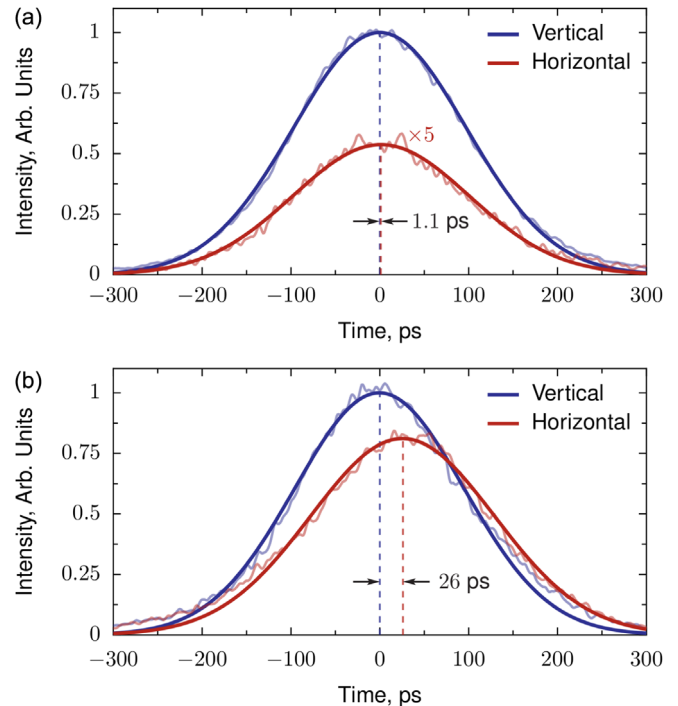
FIG. 3. Time-resolved probe envelope. (a) Streak camera traces of the incident probe horizontal and vertical polarization components, measured without plasma or pump. (b) Corresponding traces for both components after transmission through a pump-plasma system with probe detuning near the gain resonance leading to slowing of the horizontal component. A Gaussian curve is fit to all traces.
