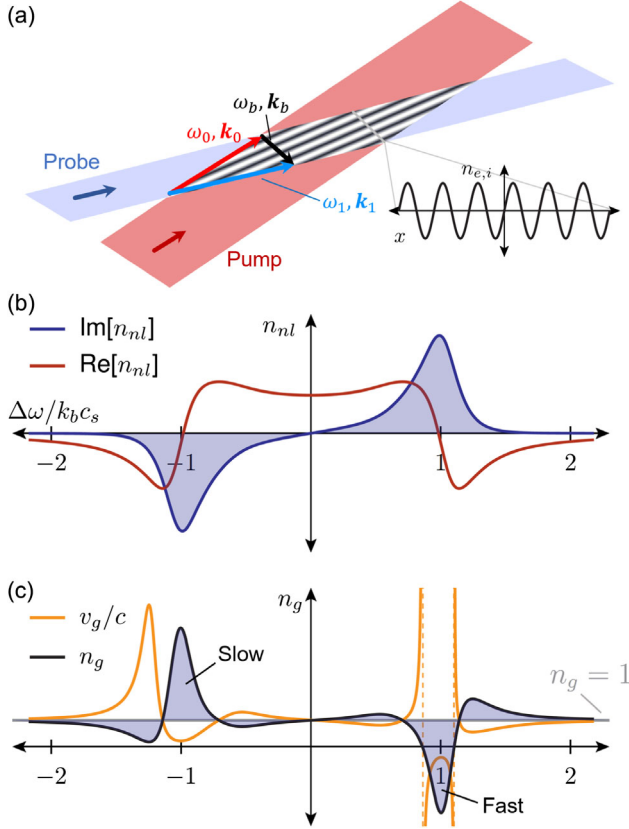
FIG. 1. Group velocity modification in plasma. (a) Schematic of the wave-mixing arrangement, with the inset graph showing ion-wave response. (b) The real and imaginary components of the nonlinear refractive index as a function of the frequency separation between pump and probe: \Delta\omega = \omega_1 - \omega_0 . (c) The corresponding group index and group velocity.
