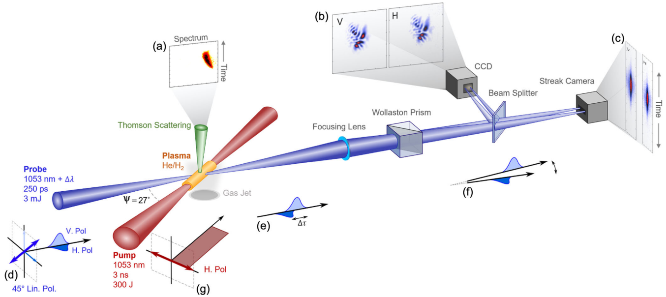
FIG. 2. Experiment schematic. The probe and pump beams interact in a plasma formed by the pump. (a) Thomson scattering of the pump beam used to measure the density and temperature. (b) CCD measures the probe focal spot and spatial distribution of gain. (c) The streak camera gives relative timing between probe polarization components and gain. (d) The incident probe is linearly polarized with H and V components. (e) Plasma introduces delay in the probe H component. (f) A Wollaston prism separates the polarization components. (g) The pump beam is polarized in the horizontal plane.
