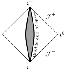
FIG. 1. Penrose diagram of the topological star. The spacetime ends as a smooth bubble at r = r_B .
