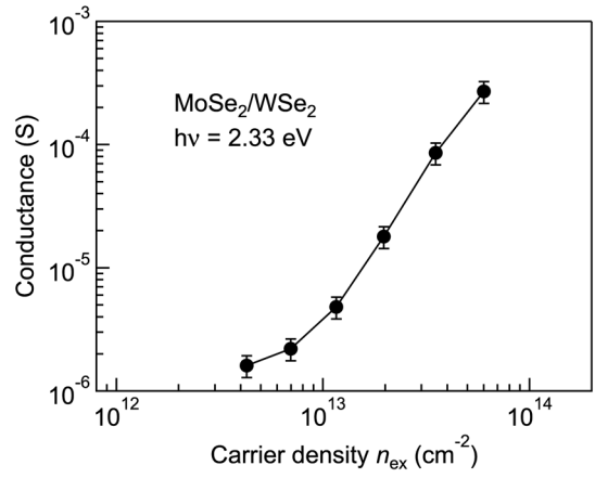
FIG. 4. Photoconductance of MoSe 2 /WSe 2 heterobilayer. Interlayer twist angle \Delta\theta > 5^\circ . Conductivity as a function of photoexcited density at h\nu = 2.33 \text{ eV} showing an insulator state to metal transition. The onset of photoconductivity is close to the Mott density, n_{\text{Mott}} \sim 1.6\text{--}3 \times 10^{12} \text{ cm}^{-2} .
