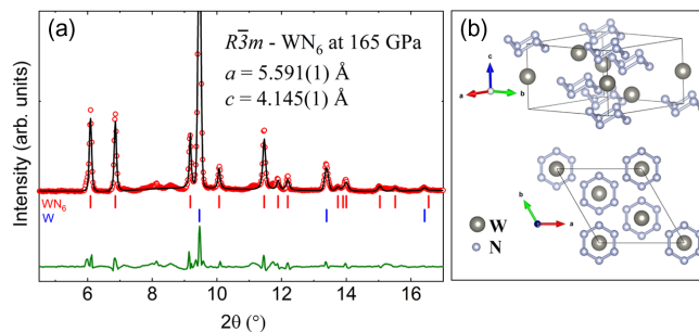
FIG. 1. Crystal structure of the \text{WN}_6 phase with the space group R\bar{3}m determined by high-pressure XRD refinement. (a) Le Bail refinement of the \text{WN}_6 phase at 165 GPa ( \lambda = 0.3344 Å) (red vertical ticks). Blue vertical ticks represent unreacted W in the bcc phase that coexists with the \text{WN}_6 . Red open circles, black line and green line represents the experimental data, the fit and the residual difference respectively. (b) Crystal structure of the \text{WN}_6 phase with the novel armchairlike \text{N}_6 rings and W atoms in between the rings along the c axis [13]. See a representative XRD image at 165 GPa shown in Fig. S5 in Supplemental Material [25].
