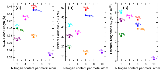
FIG. 4. Comparisons of the bond length, hardness, and toughness of the WN_6 phase with other relevant nitrides. (a) Theoretically calculated nearest N–N bond length for representative nitrides with nitrogen content ( x ) per metal atom ( WN_6 [13], MoN_6 [14], ReN_6 [14], P4/mbm WN_2 [41] and MoN_2 [42], Cmmm ReN_4 [43], Immm HfN_{10} [44], and pyrite-type PtN_2 [45]). (b) The theoretically calculated Vickers hardness ( H_v , GPa) for different nitrides with nitrogen content ( x ) per metal atom. The hardest known transition metal ( M ) nitrides ( MN_x ) are compared. (c) The calculated fracture toughness ( K_{IC} , MPa\ m^{1/2} ) for different nitrides with nitrogen content ( x ) per metal atom. Several MN_x with high toughness are selected for comparison.
