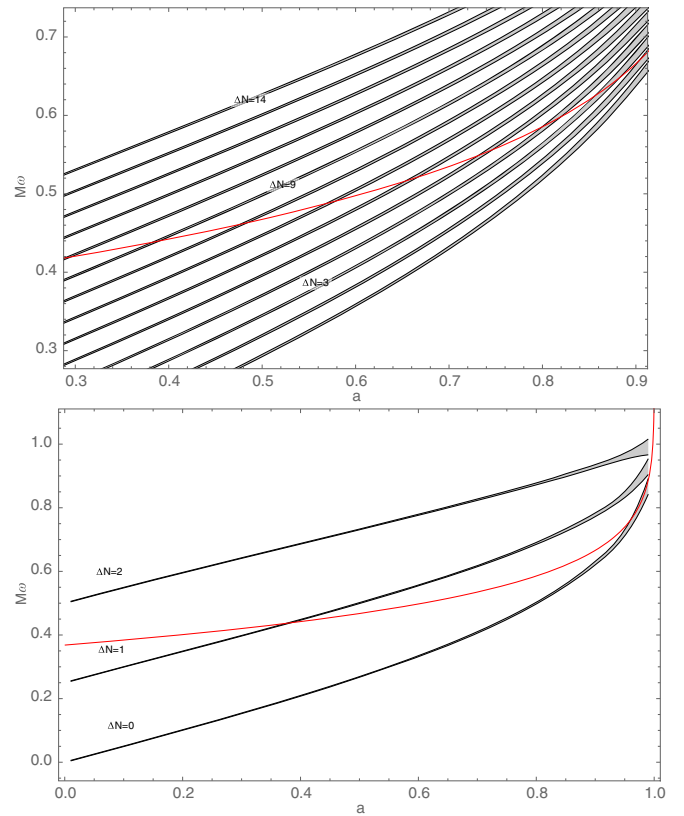
FIG. 1. BH absorption frequencies, line widths, and QNMs of spinning BHs. Black lines represent the frequencies \omega_n —defined in Eq. (4)—corresponding to the energy transitions of Kerr BHs characterized by \Delta N and \Delta j = 2 , for different values of \Delta N , as a function of the rotation parameter a . The thickness of the black lines measures the width \Gamma of the spectral lines. The upper panel shows these lines for \alpha = 4 \log 2 , while \alpha = 8\pi is shown in the bottom panel. The (real part of the) frequency M\omega_{022}(a) of the dominant QNM is shown in red. The dominant QNM will be absorbed by the BH only for values of a for which the red curve intersects one of the black lines.
