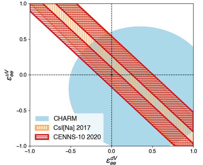
FIG. 5. 90% C.L. regions for nonstandard NSIs for a vector-coupled quark-electron interaction extracted from this argon measurement plotted together with the previous COHERENT Cs[Na] measurement [7] and the CHARM experiment [51]. The three regions shown are independent and the dashed black lines show the SM prediction.
