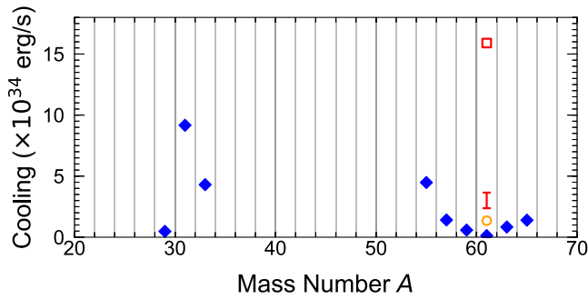
FIG. 3. The neutrino cooling contribution from individual mass chains for a neutron star crust made from rp-process ashes [14]. Predictions based on QRPA-fy (blue filled diamonds) are shown for the strongest cooling chains. For A = 61 , we also show the QRPA-fy prediction when assuming the predicted 10 keV daughter state in ^{61}\text{Cr} populated by the \beta decay of ^{61}\text{V} is in fact the ground state (red open square, see text for more discussion). The A = 61 cooling rates based on experimental transition strengths are shown without the contribution from the ^{61}\text{Cr} - ^{61}\text{V} Urca pair Letter (orange circle) and with the new data on ^{61}\text{Cr} - ^{61}\text{V} from this Letter (red error bar). Results shown are for a neutron star radius R = 12 km and a temperature T = 0.5 GK and will scale with R^2 T^5 for different physical parameters.
