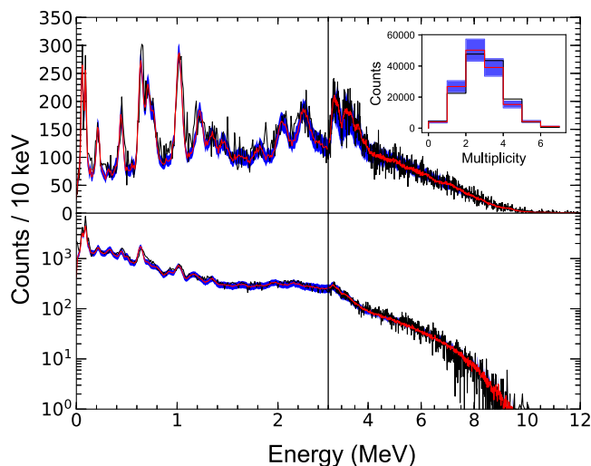
FIG. 1. Experimental (black) and fitted (red) total absorption spectrum (top), singles spectrum (bottom), and multiplicity distribution of the detector segment (inset). The 1\text{-}\sigma error band of the fit is shown in blue. The high-energy tail in the total absorption spectrum is due to a combination of the high-energy \beta particles from low-energy entry states entering SuN and \gamma -decay cascades from high-energy entry states.
