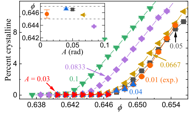
FIG. 3. The percentage of spheres in crystallites as a function of the volume fraction is shown for simulations with A = 0.03 to 0.10 rad and an experiment with A = 0.01 rad; the horizontal bars on the data points show the standard error of the mean. The results from the simulation with A = 0.05 rad and the experiment with A = 0.01 rad are remarkably similar. The inset shows that for sufficiently small A , \phi_{\text{onset}} = 0.646 \pm 0.001 .
