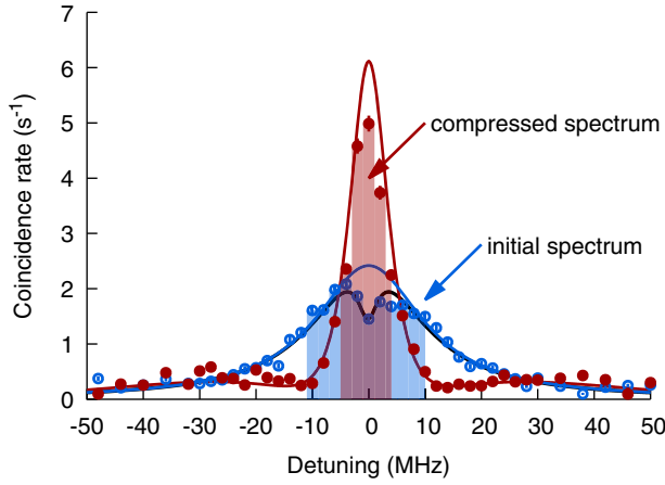
FIG. 4. Spectral profile of heralded photons before (blue) and after (red) spectral compression, obtained by measuring the photon transmission rate through the Fabry-Perot cavity at different cavity detunings. The solid lines are calculated from Eq. (5), with \Gamma_p inferred from the temporal envelope measurement of the photons from the source, and \Gamma_c by experimentally characterizing the cavity bandwidth. Shaded areas cover 50% of the total power for each spectrum.
