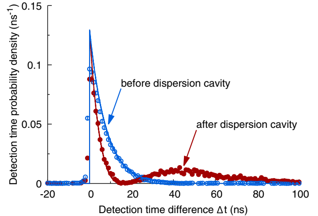
FIG. 3. Detection time distribution for the heralded photon before (open blue circles) and after (filled red dots) the dispersion cavity. We fit an exponential decay Eq. (6) to the initial time correlation (blue solid line), from which we infer the photon bandwidth \Gamma_p . The simulated temporal profile after the photon passed through the dispersion cavity [red line, calculated from Eq. (2)], matches our experimental data (filled dots) well.
