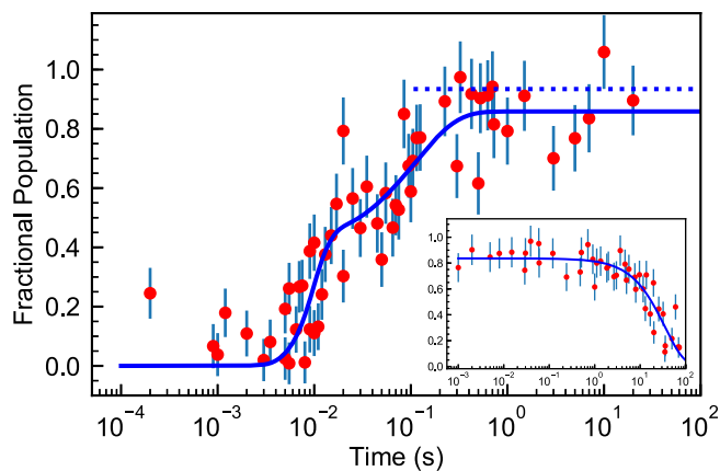
FIG. 4. Single-shot analysis of N = 0 population versus optical pumping time. Error bars account for technical noise and \text{SiO}^+ counting statistics. Since LCFMS involves difference measurements, points and error bars outside of the range of 0 to 1 are expected. The solid line is a fit to the model, and the horizontal line indicates the corrected asymptote accounting for systematic shifts. Inset: measured longevity of molecules prepared in N = 0 , after the pumping laser is turned off.
