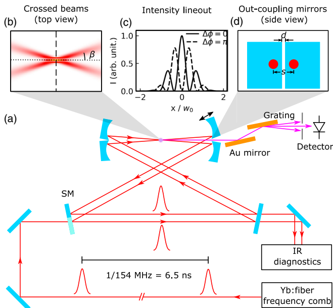
FIG. 1. (a) Schematics of the noncollinear enhancement cavity. A high-power Yb: fiber frequency comb with 154 MHz repetition rate seeds a dual-pulse fsEC whose free spectral range is set to 77 MHz. The cavity is composed of 6 mirrors: four identical curved mirrors (radius of curvature: 20 cm), one flat mirror, and one segmented mirror (SM) which is homemade by bonding a high reflector and a 1.5% transmission input coupler side by side to a flat substrate. HHG is performed at the cavity focus, where the two circulating pulses overlap temporally and spatially. The temporal delay between the two pulses is controlled via a piezoactuated mirror (indicated by black arrows). (b) Top view of the crossed beams (not to scale). Each beam forms an angle \beta with the bisecting axis (dotted line). (c) Intensity lineout at the dashed line in (b). The relative carrier phase \Delta\phi between the two beams changes the interference pattern. w_0 is the beam waist. (d) Side view of the out-coupling mirrors. The two crossed beams, separated by a distance s on the out-coupling-mirror surface, are aligned close to the edge of the mirrors with a gap size d .
