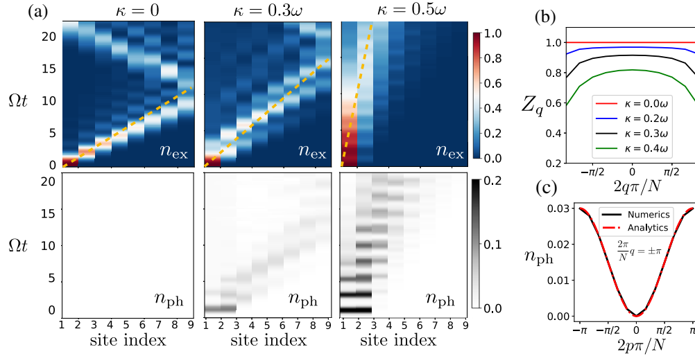
FIG. 3. Polaron dynamics. (a) Density plot of the Rydberg and phonon excitation for different values of the interaction strength \kappa/\omega . The first (second) row shows the Rydberg (phonon) density. For \kappa = 0 , i.e., in absence of interactions, a ballistic spreading of the Rydberg excitation is observed and no phonons are generated (orange dashed lines are a guide to the eye). At \kappa = 0.3\omega ( \kappa = 1.5\Omega and \omega = 5\Omega ), the propagation of the Rydberg excitation is slowed down until it almost comes to a halt (on the time scale shown) when \kappa = 0.5\omega . (b) Momentum-dependent Z factor for different values of the coupling strength. (c) Occupation number of the phonon modes in momentum space (labeled by p ) of the ground state for quasiparticle momentum (2\pi/N)q = \pm\pi and \kappa = 0.3\Omega . We compare the analytical result of Eq. (9) with numerical data obtained using exact diagonalization on a system up to N = 12 sites.
