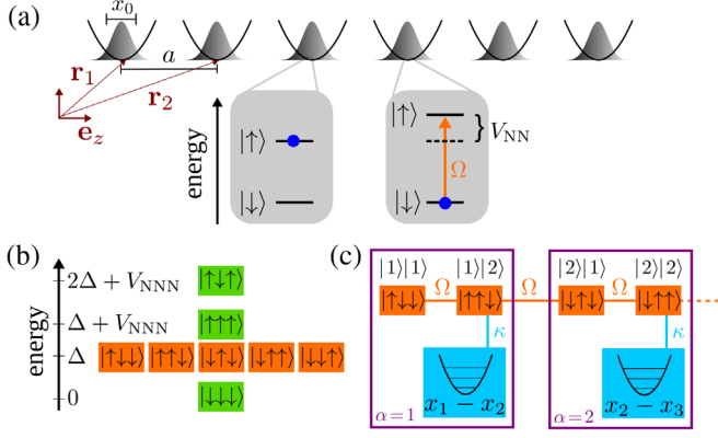
FIG. 1. Setting. (a) Schematic representation of the Rydberg quantum simulator. The internal degrees of freedom of each trapped atom are approximated by a two-level system. Here, \Omega is the Rabi frequency of the excitation laser that is detuned from the atomic transition by an energy \Delta , and the interaction between nearest neighbors is parametrized by V_{\text{NN}} . The atoms are confined in a one-dimensional chain of harmonic traps, where a is the lattice spacing and x_0 represents the harmonic oscillator length. (b) Hilbert space representation in the facilitation regime. The many-body configurations at energy \Delta are resonant and effectively decoupled from the rest of the Hilbert space. V_{\text{NNN}} is the interaction among next-nearest neighbors in Rydberg states. (c) Hilbert space defined by the effective lattice of resonant many-body states and their coupling to harmonic oscillator modes. Only states with two contiguous Rydberg excitations are coupled to the (relative) vibrational mode of the traps.
