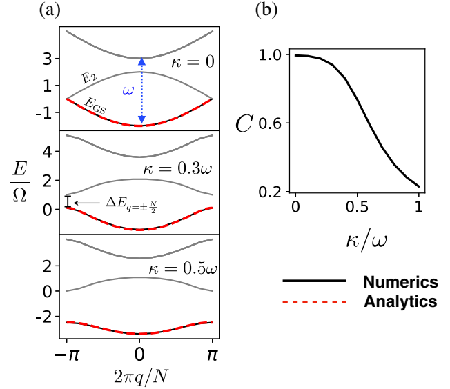
FIG. 2. Band structure. (a) Comparison between the analytical form Eq. (8) and numerical calculations obtained for N = 12 and truncation of the maximum number of phonons per site to 3. The noninteracting bands form a ladder with spacing \omega . As the interaction between the lattice and phonons increases, the band degeneracies at the edges are lifted and the ground state band is flattened. (b) Curvature C of the ground-state band computed for quasiparticle momentum q = 0 , numerical results.
