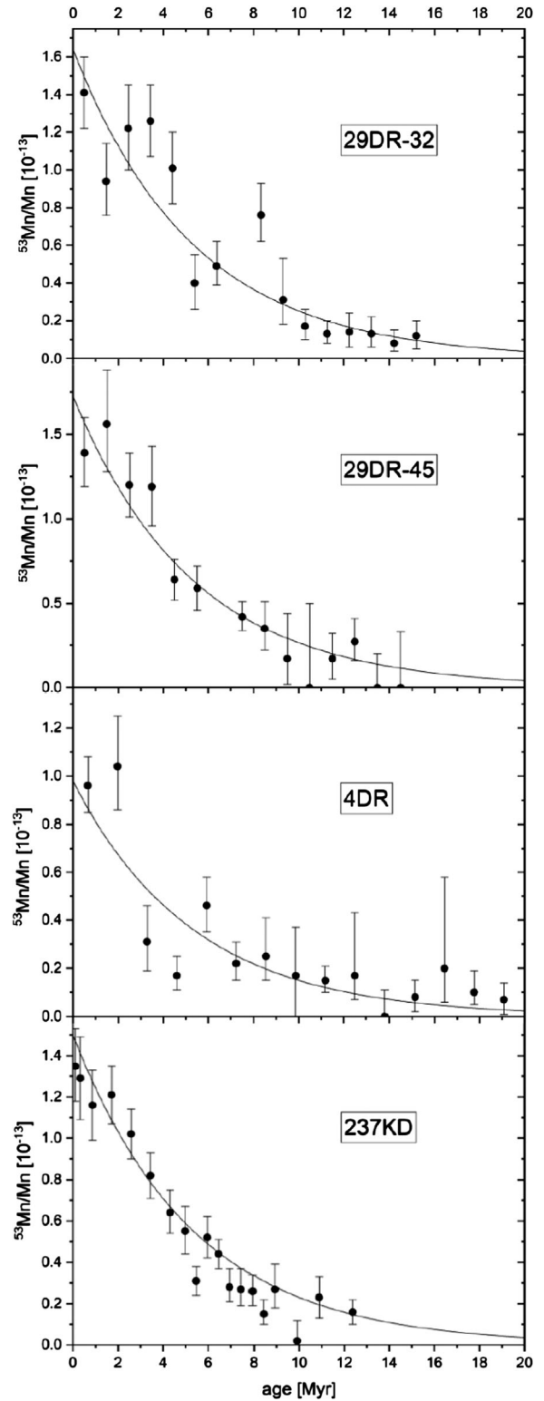
FIG. 1. Shows the measured isotope ratios ^{53}\text{Mn}/\text{Mn} at different depths/ages in the crusts. Top to bottom are for the four crusts from the Pacific: the two from Midway atoll, (29DR-32 and 29DR-45), one from the Donizetti ridge (4DR) and one from Central Pacific (237KD). Error bars for small event numbers were calculated following the prescription of Feldman and Cousins [34]. The 1\sigma limits are drawn.
