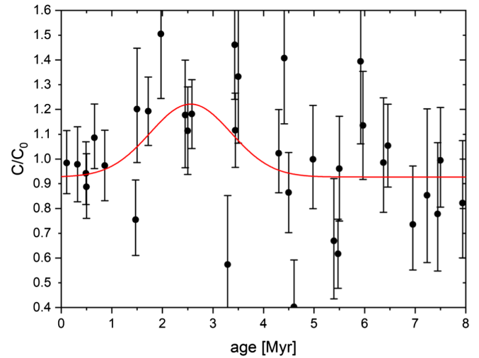
FIG. 2. Merged ^{53}\text{Mn}/\text{Mn} ratios ( C/C_0 ) from the different crusts at the time of incorporation. The red curve is the result of a fit of a Gaussian with fixed width \sigma = 0.8 Myr.
