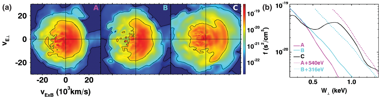
FIG. 4. Reduced electron distribution functions in the background E \times B (low pass filtered fields below 1 Hz) drift frame showing nongyrotropic perpendicular heating and direct acceleration by the LHDW potential. (a) Distributions ABC [corresponding to the data points marked in Fig. 3(d)] in the v_{E \times B} - v_{E\perp} plane, where v_{E \times B} and v_{E\perp} are along the E \times B and perpendicular electric field directions, respectively. (b) Phase-space densities of the reduced distributions ABC as a function of the perpendicular energy W_{\perp} along the direction of v_{E \times B} . The dotted magenta (light-blue) curve is distribution A (B) shifted by the potential energy difference between time A (B) and time C, and agrees with distribution C within uncertainties ( \pm 150 eV given by the instrument's energy bin width and/or the potential energy change over the distribution sampling time).
