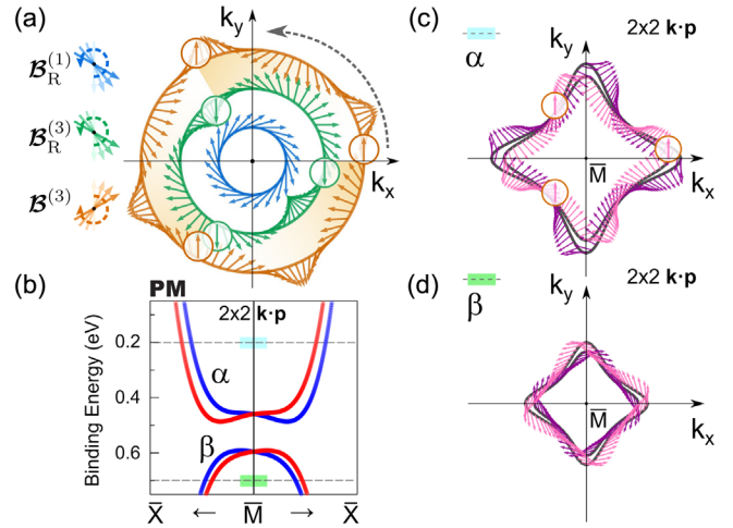
FIG. 3. (a) Effective spin-orbit magnetic fields \mathcal{B}_R^{(1)} ( R^{(1)} effect, blue arrows), \mathcal{B}_R^{(3)} (‘‘heavy-hole’’ R^{(3)} effect, green arrows), and \mathcal{B}_R^{(3)} ( R^{(3)} effect for the state \alpha , orange arrows) as a function of polar angle \varphi_{\mathbf{k}} . The legends on the left show the rotation direction of the vectors \mathcal{B}_R^{(1)} , \mathcal{B}_R^{(3)} , and \mathcal{B}_R^{(3)} with the anticlockwise rotation of \mathbf{k} (gray dashed arc arrow). (b) Band structure of the states \alpha and \beta by the Hamiltonian (1) presented by red ( S_y > 0 ) and blue ( S_y < 0 ) bands. Graphs (c) and (d) show spin-resolved CECs by the \mathbf{k} \cdot \mathbf{p} model at the binding energy of 0.2 and 0.7 eV, respectively [indicated by dashed gray lines in graph (b)], with the S_{\parallel} orientation shown by pink (purple) arrows for the inner contour and by purple (pink) for outer contour of the state \alpha ( \beta ).
