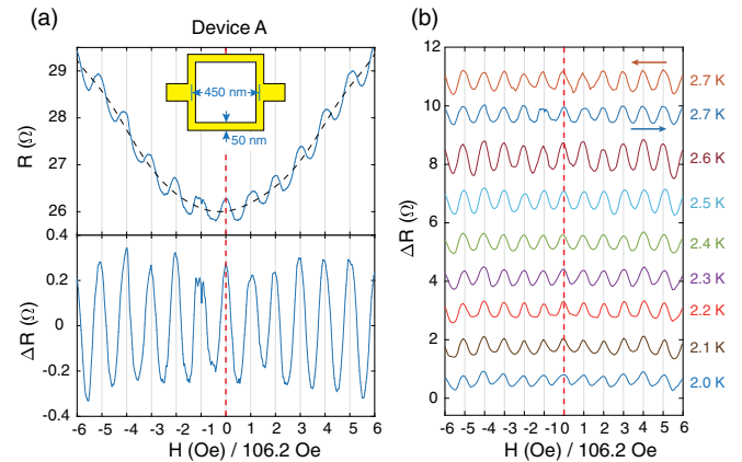
FIG. 2. Little-Parks effect of device A. (a) Upper panel: resistance as a function of applied magnetic field at 2.7 K. The red vertical dashed line denotes the zero field and the gray lines denote the fields at n\Phi_0 . Device A has an enclosed area of 450 \times 450 nm, which leads to an expected oscillation period of 102.1 Oe. The black dashed line is the fitted background curve. Lower panel: Little-Parks oscillation after subtraction of the background. (b) Temperature dependence of Little-Parks oscillations from 2 to 2.7 K. The two curves at 2.7 K are obtained when sweeping the magnetic field in opposite directions.
