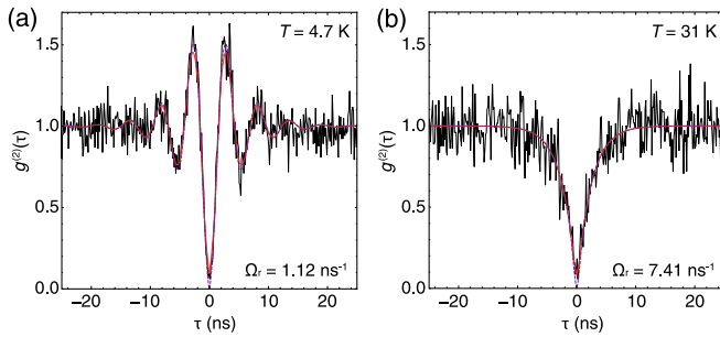
FIG. 3. Measured g^{(2)}(\tau) taken from the DBT molecule at (a) 4.7 and (b) 31 K. Black shows the experimental data. Red solid lines show the theoretical model convolved with a Gaussian function to account for the detector timing jitter and purple dashed lines show the model without convolution.
