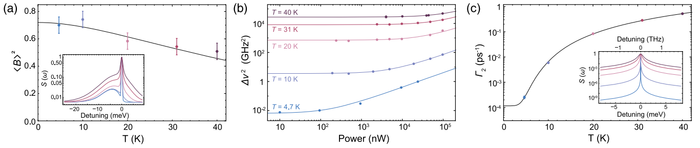
FIG. 2. (a) Debye-Waller factor \langle B \rangle^2 for varying temperature. The solid line shows the theory. The inset shows the calculated spectrum of the ZPL and sideband at temperatures where the data was taken. (b) Squared linewidths extracted from fluorescence excitation spectra for varying power at different temperatures. Lines are fits to \Delta\nu^2 = (\Gamma_2/\pi)^2(1 + S) . (c) Experimental values of \Gamma_2 found from the fits in (b), plotted together with prediction from the theoretical model (solid line). The inset shows the calculated Lorentzian ZPL for temperatures at which the data were taken.
