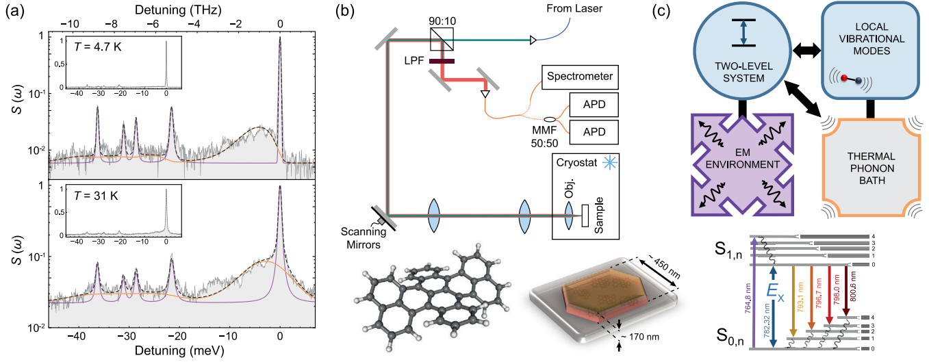
FIG. 1. (a) Single DBT molecule emission spectra taken at 4.7 K (top) and 31 K (bottom). Black-dashed lines show the full theoretical model and gray-solid lines show experimental data. The theoretical spectrum showing only the zero-phonon line and local vibrational mode peaks is shown in purple [cf. Eq. (3)], while the broad phonon sideband contribution is shown in orange [Eq. (4)]. The insets show the spectra on a linear scale. (b) Simplified schematic of the confocal microscope. Dark green is the pump light, and red is the fluorescence. 90% reflection, 10% transmission beam splitter (90:10); Objective lens (Obj); long-pass filter (LPF); 50% reflection, 50% transmission multimode fiber beam splitter (MMF 50:50); avalanche photodiode (APD). The nanocrystal sample (bottom right) consists of DBT (bottom left) embedded in anthracene. (c) Open quantum system model of a single DBT molecule. The system (blue) contains a two level electronic system (TLS) coupled to a discrete set of vibrational modes and an electromagnetic environment. The thermal phonon bath originates from the nanocrystal and is coupled separately to both system elements. The arrows connected to the TLS represent a non-Markovian interaction including feedback. The schematic energy level diagram shows the ground S_0 and excited S_1 electronic singlet states with energy splitting E_X , and local vibrational modes, all broadened by the thermal phonon environment.
