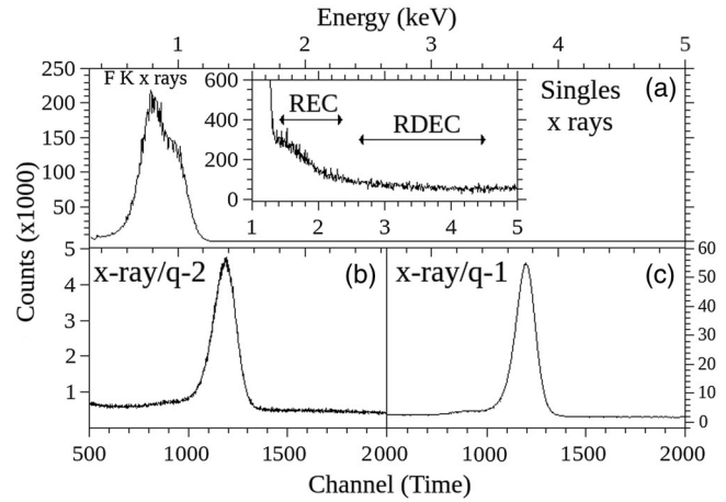
FIG. 2. Sums of collected (a) x-ray singles events, (b) x-ray/doubly charge-changed ( q-2 ), and (c) x-ray/singly charge-changed ( q-1 ) coincidence events for 2.11 MeV/u F^{9+} + N_2 .
