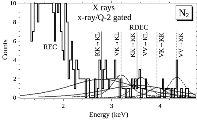
FIG. 5. X-ray spectrum obtained from events sorted on the x-ray/q-2 coincidence spectrum [Fig. 2(b)] for 2.11 MeV/u F^{9+} incident on N_2 . The smooth curves under the RDEC region show the calculated Compton profiles of the transitions arbitrarily normalized to the data. The following scheme is used based on the initial state of the transition: VV is indicated by the short dashed lines, VK by the long dashed lines, and KK by the solid lines.
