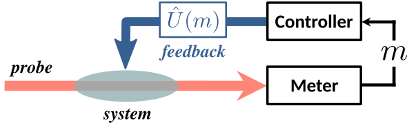
FIG. 1. Schematic for a measurement-and-feedback-based quantum simulator. A quantum system undergoes weak measurements, yielding an outcome m . This is then fed back to the system via a quantum control operation \hat{U}(m) .
