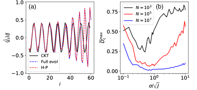
FIG. 2. (a) Time evolution of \langle \hat{J}_z \rangle / J for regular dynamics. Dashed blue: full quantum evolution, dashed red: H-P approximation, black: classical KT. (b) Maximum distance to the corresponding classical trajectory averaged over several initial conditions \bar{D}_c^{\max} as a function of the measurement resolution. An optimal value of \sigma exists around \sigma \sim \sqrt{J} . For both cases, parameters are: k = 1.5 , N = 10^3 , \sigma = 0.9\sqrt{J} .
