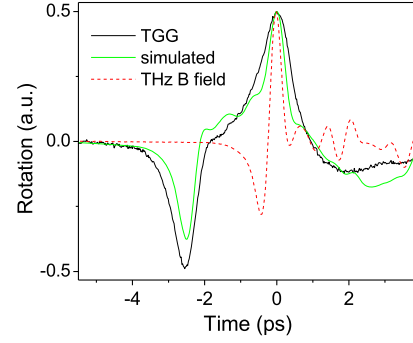
FIG. 4. The magneto-optic Faraday rotation of a terbium gallium garnet crystal and the simulated signal in which the velocity mismatch between the THz and optical pulses is taken into account (see text). The dashed line shows the THz magnetic field.
