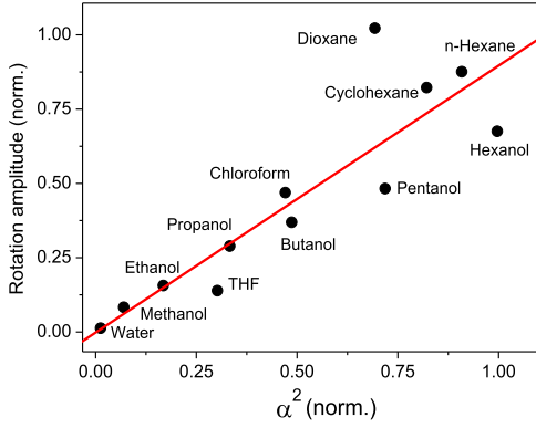
FIG. 5. Peak-to-peak amplitude of the Faraday rotation signal of liquids is plotted vs the square of the average molecular polarizability of liquids, taken from the following references: water [42], cyclohexane [43], chloroform, methanol, ethanol, propanol, butanol, pentanol, hexanol, n -hexane, dioxane [38], and tetrahydrofuran (THF) [44].
