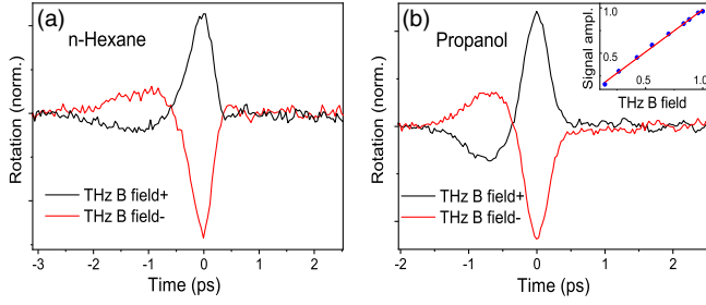
FIG. 3. Faraday rotation of n -hexane (a) and propanol (b) scales linearly with the applied THz magnetic field. In both samples the measured signal flips sign, by 180^\circ phase shift of the THz magnetic field. Inset in panel (b) shows the fluence dependence of the peak-to-peak amplitude of the rotation signal of propanol.
