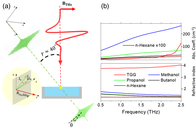
FIG. 1. (a) A femtosecond optical pulse is mixed under a wide angle of \sim 40^\circ with a single cycle linearly polarized THz pulse on liquids. The optically induced instantaneous polarization acts as a current burst \mathbf{J}_e(t) . This current is bent by the THz magnetic field in the plane perpendicular to the optical pulse propagation direction. The deflected component of the current, i.e., \mathbf{J}_H(t) causes the rotation of the optical pulse polarization. The liquids are held in an open-top bucket. In this configuration, the THz pulse impinges the sample vertically. (b) THz absorption and refractive index of some of the samples used in this study. For the TGG crystal, data is obtained from our THz time-domain spectrometer. The refractive index and absorption coefficient of methanol [24], butanol, propanol [25], and n -hexane [26] are calculated from their dielectric permittivity and loss spectra of the cited references.
