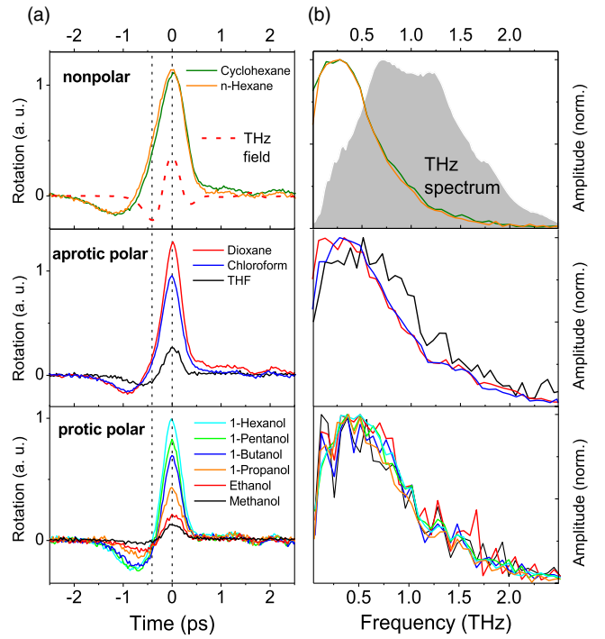
FIG. 2. (a) Faraday rotation of a series of molecular liquids at room temperature. Nonpolar, cyclohexane (dark green) and n -hexane (red); aprotic polar, dioxane (pink), chloroform (blue), tetrahydrofuran (THF, black); protic polar, 1-hexanol (cyan), 1-pentanol (green), 1-butanol (blue), 1-propanol (pink), ethanol (red) and methanol (black). The measured signals resemble the THz waveform (dashed line). (b) The Fourier spectra of the signals in panel (a). The gray area shows the amplitude spectrum of the THz pulse.
