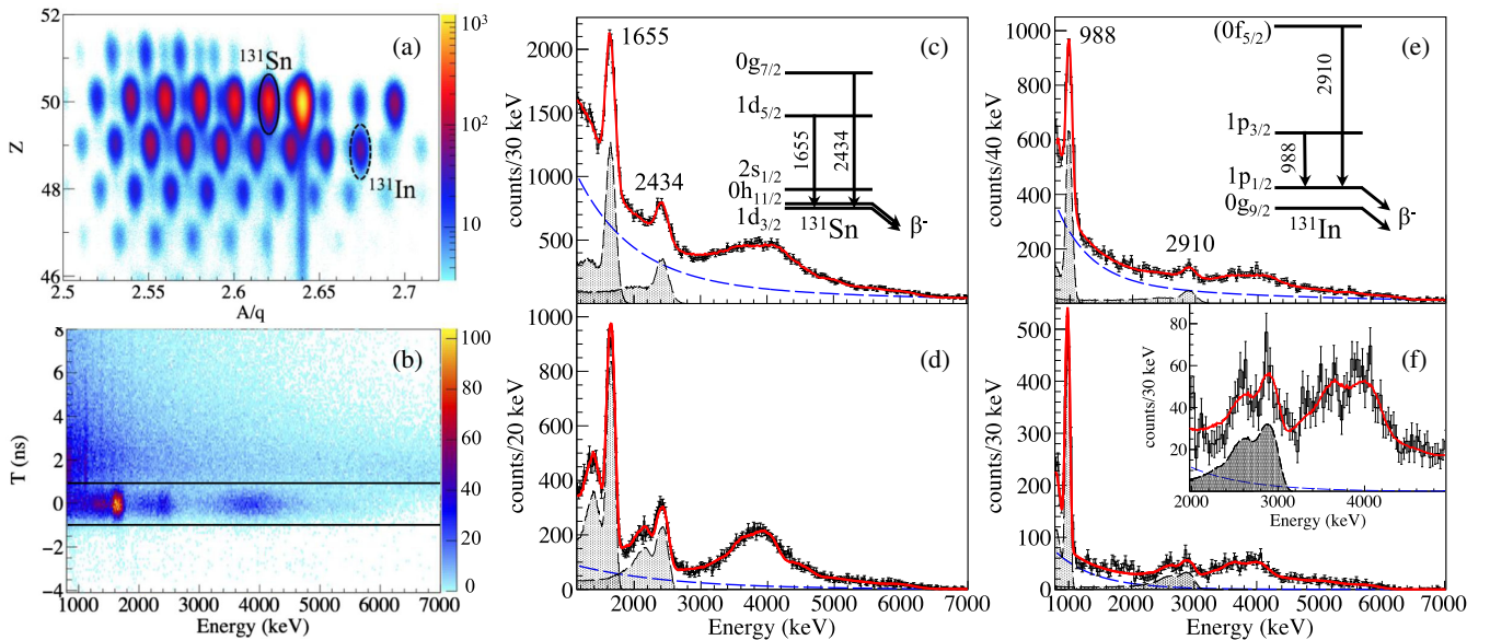
FIG. 1. (a) ZeroDegree particle identification plot for the ^{132}\text{Sn} beam impinging on the helium reaction target. (b) \gamma -ray energy vs time matrix for ^{131}\text{Sn} measured with the \text{LaBr}_3 detectors. Doppler-corrected \gamma -ray spectra of ^{131}\text{Sn} populated via one-neutron removal from ^{132}\text{Sn} measured with (c) the NaI and (d) the \text{LaBr}_3 detectors. (e), (f) Same as (c), (d) for ^{131}\text{In} populated via one-proton removal. In (c)–(f) the fit to the experimental spectrum (red solid line) is the sum of the background (blue dashed line) and the simulated response functions for the observed transitions (filled curves). In (c), (e) only events with multiplicity M_\gamma = 1 are considered in order to reduce the background. The insets in (c) and (e) show the level schemes of ^{131}\text{Sn} and ^{131}\text{In} , respectively.
