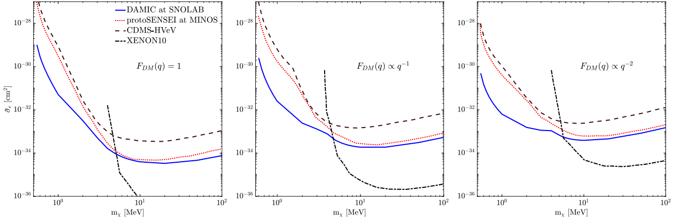
FIG. 3. 90% C.L. upper limits on the DM-electron free scattering cross section \bar{\sigma}_e as a function of DM mass m_\chi for F_{DM} \propto q^{-n} ( n = 0, 1, 2 ) obtained by DAMIC at SNOLAB (solid line). Current best limits from protoSENSEI at MINOS [18,19], CDMS-HVeV surface run (dashed line) [20], and an analysis of the XENON10 data (dashed-dotted line) [21] are also shown for comparison.
