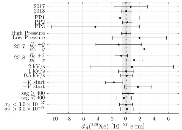
FIG. 2. Comparison of EDM measurements for both the 2017 and 2018 campaigns grouped by cell, cell pressure, \hat{B}_0 direction, HV ramp rate, HV start polarity, HV segment length, and EDM uncertainty \sigma_{d_i} < 3.00 \times 10^{-27} e cm (five subruns) or \sigma_{d_i} > 3.00 \times 10^{-27} e cm (75 subruns). The shaded area shows the result given in Eq. (2).
