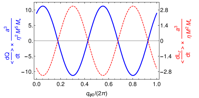
FIG. 1. Average change rate of the Carter constant (solid, blue) and angular momentum along the z direction (dashed, red) as a function of q_{\phi 0} for the case with a = 0.99 (see Table I). Both \langle dQ/dt \rangle and \langle dL_z/dt \rangle are normalized by \epsilon to remove the associated linear dependence and powers of M to be dimensionless.
