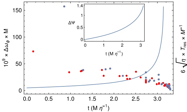
FIG. 2. Evolution of the difference in \omega_{\phi} between inspirals with and without resonant \Delta J_i (blue curve), and illustration of resonances encountered during inspiral (dots). We take the central black hole to have M = M_{\text{SgrA}^*} ; both the inspiraling body \mu and the perturbing tidal source M_* are 10 M_{\odot} , and the tidal source is at separation R = 4.3 \text{ AU} . The orbits start at the resonance point q_{\phi 0} = 0.33 in Fig. 1; the final time is the plunge. Red and blue dots show the resonance duration T_{\text{res}} for resonances with \{|m|, |k|, |n|\} \leq 5 ; blue dots indicate m = \pm 2 . (The right-hand vertical axis has the same scale as the left.) The tightly bunched dots in the lower right illustrate how the system passes rapidly through multiple tidal resonances in quick succession as plunge is approached. (Inset) The associated accumulated phase shift.
