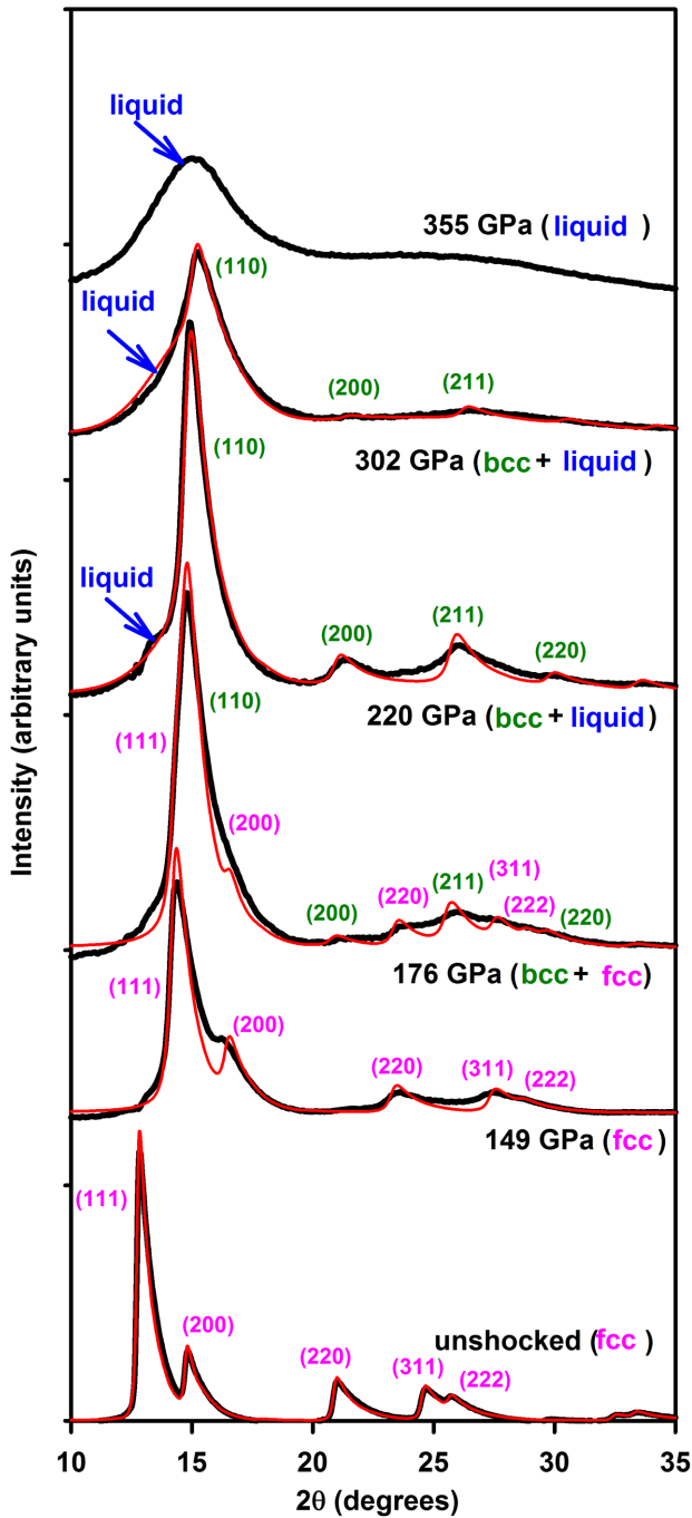
FIG. 2. Representative measured and simulated XRD line profiles for ambient and laser-shocked gold samples. The thick black lines are measured line profiles with background subtracted. For shocked state line profiles, the contribution from unshocked Au was also subtracted. The thin red lines are simulated line profiles using fcc and/or bcc lattice parameters that give the best match between simulated and measured profiles. Simulated line profiles for shock stresses 220 GPa or higher included a contribution from liquid scattering [25]. No simulation is shown for the 355 GPa experiment since crystalline peaks were not observed. Peaks corresponding to the fcc (bcc) structure are listed with pink (green) indices and features due to liquid scattering are identified by blue arrows.
