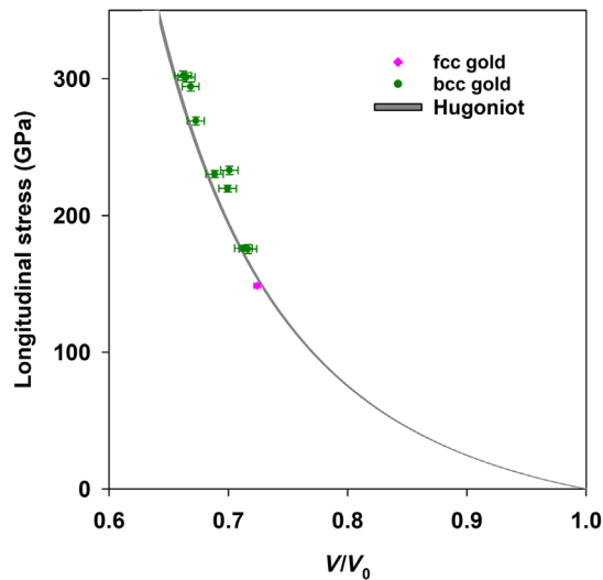
FIG. 3. Stress vs volume for shock-compressed gold. The pink diamond shows the volume for fcc Au at 149 GPa. The green circles show the volumes for bcc Au. The volumes were determined from the measured XRD data; the stresses were determined from the measured velocity profiles at the Au/LiF interface [25]. The gray band is the Hugoniot curve based on continuum measurements from Refs. [12,26,27]; the uncertainty in the curve is indicated by the width of the band.
