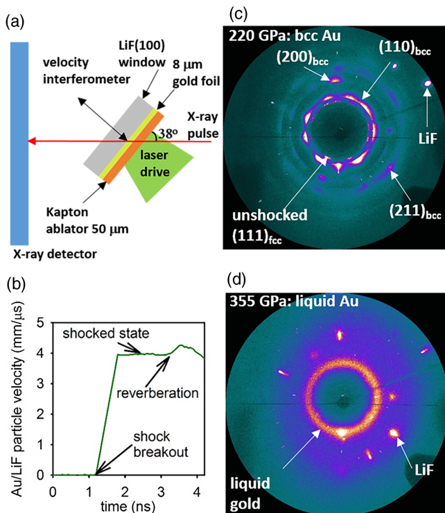
FIG. 1. Experimental configuration and representative results. (a) Schematic of the configuration for in situ continuum and x-ray diffraction measurements in laser shocked Au. (b) Representative measured Au/LiF window interface velocity history showing a flat-topped shocked state. (c) Representative XRD pattern measured for Au shock compressed to 220 GPa. Diffraction rings corresponding to the bcc structure are dominant. However, ambient fcc diffraction rings remain visible since \sim 15\% of the material was still unshocked at the time of the x-ray diffraction measurement. (d) X-ray diffraction pattern showing a liquid scattering ring for Au fully shocked to 355 GPa.
