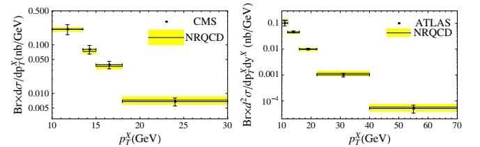
FIG. 2. The differential cross sections of prompt X(3872) production as measured by CMS [17] (left panel) and ATLAS [18] (right panel) are compared with our NLO NRQCD results based on the new fit (solid lines). The yellow bands indicate the theoretical uncertainties.
