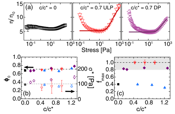
FIG. 3. (a) Relative viscosity as a function of stress, fit to Eq. (1) [5,10] for representative suspensions without polymer, with normalized polyacrylamide concentration in the free volume c/c^* = 0.7 ULP, and with c/c^* = 0.7 DP. (b),(c) Fit parameters extracted from Eq. (1) as a function of c/c^* . Dashed lines are guides for the eye at (b) \phi_0 = 0.71 , \sigma^* = 100 Pa, (c) f_{\max} = 1 . Samples in the shaded region ( f_{\max} > 0.8 ) exhibited N_1 > 0 .
