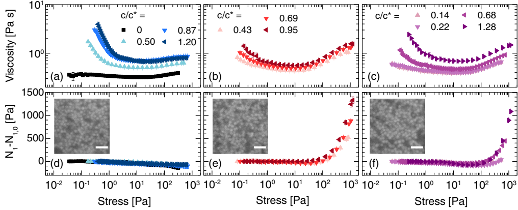
FIG. 1. (a)–(c) Viscosity and (d)–(f) corrected N_1 as a function of shear stress for \phi = 0.40 suspensions with various free-volume concentrations of polyacrylamide c/c^* , normalized by the overlap concentration c^* . Polymers (a),(d) USP; (b),(e) ULP; (c),(f) DP. Insets: Micrographs of quiescent suspensions with c/c^* = (d) 0.5 USP, (e) 0.7 ULP, and (f) 0.7 DP. Scale bars: 5 \mu\text{m} .
