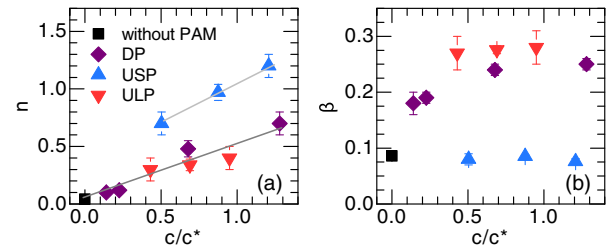
FIG. 2. Power-law (a) shear-thinning ( n ) and (b) shear-thickening ( \beta ) exponents as a function of normalized polyacrylamide (USP, ULP, DP) concentration in the free volume c/c^* for \phi = 0.40 suspensions. Gray lines are guides for the eye.
