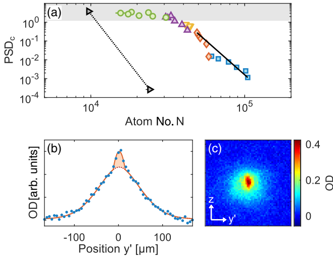
FIG. 3. (a) Classical phase-space density PSD_c as a function of remaining atom number N . The cooling is very efficient until PSD_c \sim 1 is reached. The black symbols denote the performance of the same sequence with the initial atom number reduced by a factor 5. The final atom number is only reduced by a factor 2, indicating a density limit in the cooling. The solid (dashed) black line indicates the S1-S2 (S1-X3) path with an efficiency \gamma = 7.2 ( \gamma = 11 ) for each case. (b) Line optical density (dots) of the cloud in time of flight along the y' direction (slightly rotated from the y direction in the x - y plane, see Supplemental Material [27]). The data are taken after 1.6 s of cooling and fitted with a g_{5/2} Bose distribution with a Thomas-Fermi distribution superimposed (orange line). The shaded area indicates the condensed fraction. (c) False-color image of the optical density (OD) of the same cloud (before integration along the vertical direction), showing the anisotropic expansion of the condensed fraction in the center.
