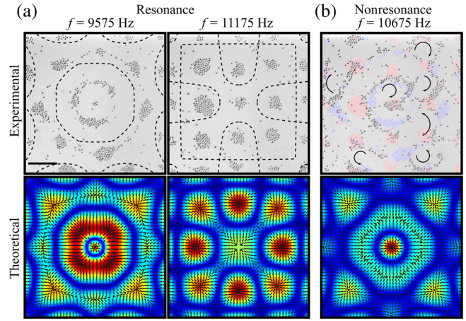
FIG. 2. (a) Experimental and theoretical resonant patterns: in the experimental figures (first row), the black dashed lines are overlaid for better visualization of the nodal lines. In the theoretical figures (second row), the time-averaged horizontal effective weight \langle W_{\parallel} \rangle (arrows) is overlaid on the theoretical vibration amplitude \xi , where the force points towards the antinodes. (b) Experimental and theoretical nonresonant patterns: in the experimental figure, arrows show the vortexlike motion path. It follows that the adjacent resonant patterns, which are underlaid in the experimental figure, affect the path of the vortexlike motion. Scale bar, 10 mm.
