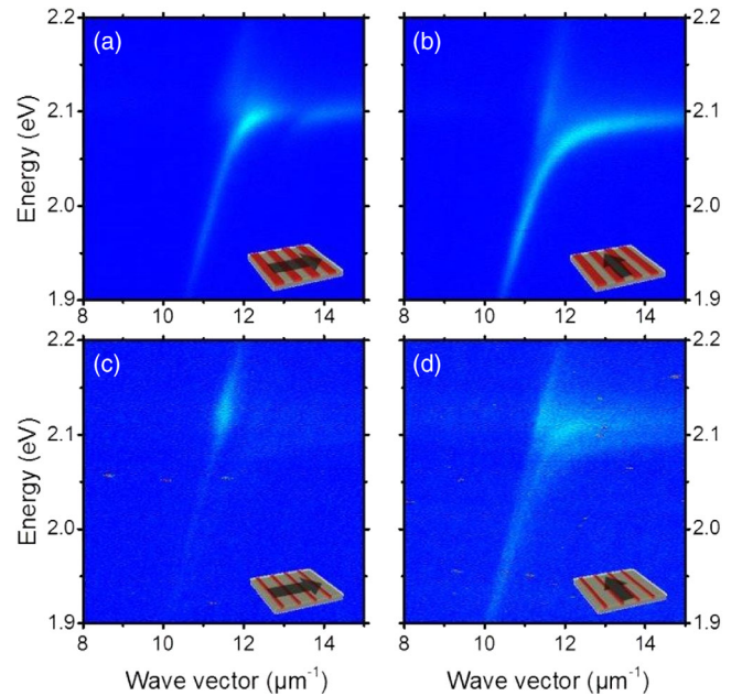
FIG. 4. Anisotropic emission dispersion properties of polaritonic metasurfaces with two different filling factors. (a),(b) Filling factor 1/2 (the stripe width is 2.5\ \mu\text{m} , and the period is 5\ \mu\text{m} ). (c),(d) Filling factor 1/10 (stripe width 1\ \mu\text{m} ).
