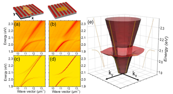
FIG. 2. Dispersion relations measured for a 5 \mu\text{m} period pattern with the propagation direction (a) parallel to the stripes and (b) perpendicular to the stripes, as well as corresponding calculated dispersion relations (c),(d). (e) Two-dimensional experimental dispersion surface reconstructed across all propagation directions (from directions orthonormal to the stripes k_x to directions parallel to the stripes k_y ). For clarity, the region of wave vectors with magnitudes lower than 10 \mu\text{m}^{-1} is removed.
