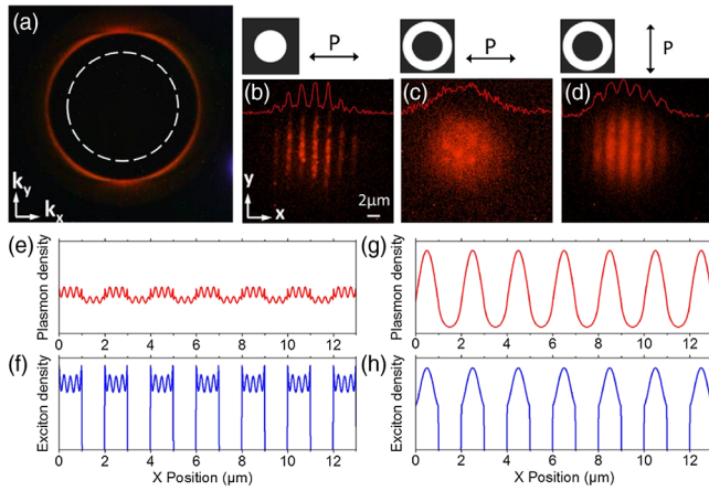
FIG. 3. Emission properties of polaritonic metasurface with a 2\ \mu\text{m} period, with stripes oriented along the y direction. (a) Fourier space image of the luminescence. The white dashed circle limits the Fourier space filtering areas used in (b)–(d) for direct space imaging. (b) Direct emission image of the incoherent states. (c),(d) Direct emission image associated with large wave vectors with a polarization direction perpendicular (c) and parallel (d) to the stripes. The intensity profile at the center of the image along the x axis is plotted as a red line on top of each image. (e)–(h) Plasmon and exciton density of the calculated low-energy polariton wave function at resonance for propagation perpendicular (e),(f) and parallel (g),(h) to the stripes.
