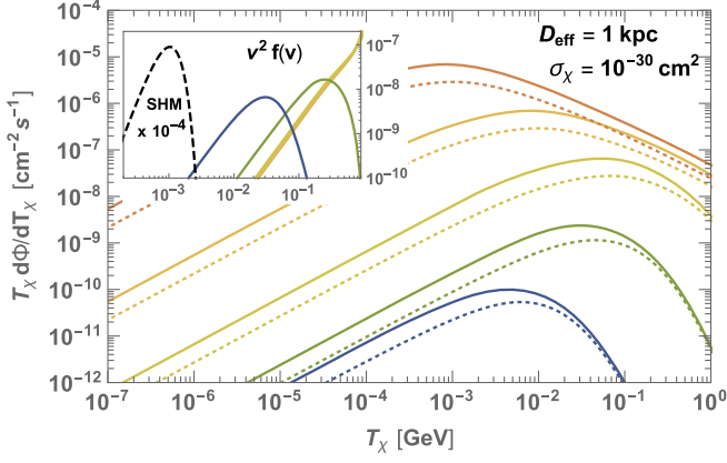
FIG. 1. Expected flux of CRDM for different DM masses m_\chi = 0.001, 0.01, 0.1, 1, 10 GeV (from top to bottom). Dotted lines show the contribution from CR proton scattering alone. The flux is directly proportional to the effective distance D_{\text{eff}} and the elastic scattering cross section \sigma_\chi , chosen here as indicated. (Inset) Compares the corresponding 1D velocity distributions f(v) , in units where c = 1 , to that of the standard halo model (SHM) (dashed line).
