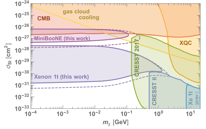
FIG. 2. Constraints on spin-independent DM-nucleon scattering imposed by the XENON-1T and MiniBooNE experiments. Solid (dashed) lines assume a CR density that equals, on average, the local value out to a distance of 1 kpc (10 kpc). We compare our limits to those deriving from cosmic microwave background (CMB) observations [40], gas cloud cooling [38], the x-ray quantum calorimeter experiment (XQC) [39], and a selection of direct detection experiments [43–45] after taking into account the absorption of DM in soil and atmosphere [33].
