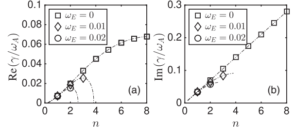
FIG. 2. Real (a) and imaginary (b) parts of \gamma evaluated from Eq. (8) with q \approx 5 , \varepsilon = 1/3 , r_1/a = 0.95 , \Omega_1/\omega_A = 5 \times 10^{-2} , \omega_I/\omega_A = 3 \times 10^{-3} , \beta_1 = 0.3\% , and \delta q = 0.1 .
