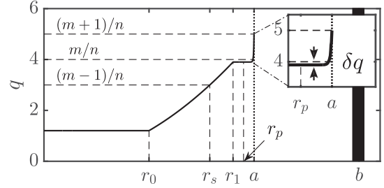
FIG. 1. Example of a model safety factor profile employed in our analysis. Note the (m+1)/n resonance at the plasma boundary mimicking the separatrix.
