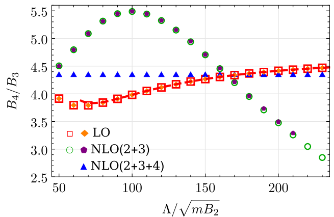
FIG. 1. The tetramer binding energy in units of the trimer ground-state energy is plotted as function of the cutoff in units of \sqrt{mB_2} . LO and NLO results without a four-body force from the FY (orange diamonds and purple pentagons) and SVM (red squares and green circles) methods are in very good agreement. They are compared to the result calculated directly [43] from the PCKLJS potential, which coincides (by construction) with the NLO result with a four-body force (blue triangles). The red dashed curve is a fit in powers of \Lambda^{-1} .
