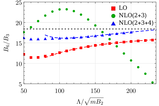
FIG. 3. The hexamer ground-state energy is plotted as function of the cutoff in the same units as Fig. 1. Symbols are as in Fig. 2.
