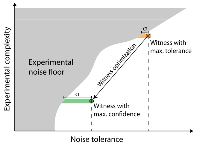
FIG. 1. Complexity of the measurement settings vs noise tolerance of the witness. In any experiment, the measurement settings introduce an experimental noise floor (gray area), which increases with the measurement complexity. The optimal theoretical witness (orange square) has the highest noise tolerance, but it demands intricate and often unfeasible measurements. The optimal experimental witness (green circle) requires reduced measurement complexity, at the cost of having a lower noise tolerance. The goal is to maximize \sigma (the shaded green or orange area), which represents the measurement confidence, given by the distance between the noise floor and the witness noise tolerance. Such maximization provides the highest confidence to measure a negative expectation value of the witness.
