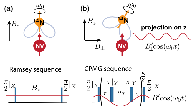
FIG. 1. Vector magnetometry. (a) The magnetic field component B_z along the NV axis can be measured by a Ramsey sequence. Without the transverse field, there is no S_z I_{\perp} interaction (light blue) between the NV ^{14}\text{N} nuclear spin and the electronic spin, that only feels a static field. (b) The transverse field modifies the hyperfine coupling, introducing an effective S_z I_{\perp} coupling at the position of the NV. As the nuclear spin precesses at its Larmor frequency \omega_0 , the effective field felt by the NV is now an oscillating ac field with amplitude B'_{\perp} proportional to B_{\perp} , that can be measured by a CPMG sequence of N \pi pulses separated by 2\tau = \pi/\omega_0 .
