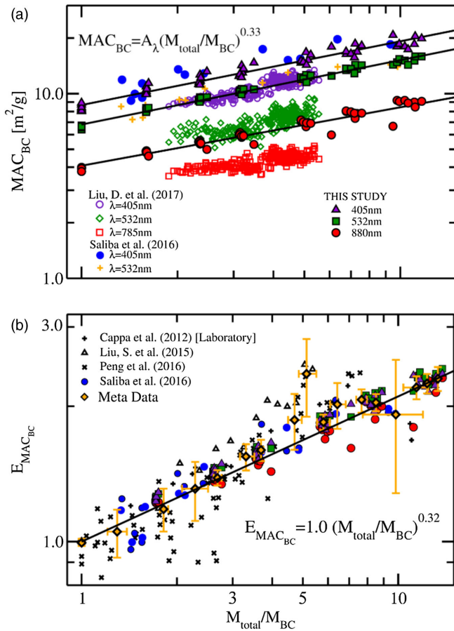
FIG. 2. The 1/3 scaling laws for BC mass absorption cross section ( MAC_{BC} ) and enhancement of MAC_{BC} ( E_{MAC_{BC}} ). The MAC_{BC} vs total coated aggregate mass divided by its bare BC mass ( M_{total}/M_{BC} ) at wavelengths \lambda = 405, 532, and 880 nm is shown in (A). At all \lambda , MAC_{BC} scales with a power-law exponent of 0.33 \pm 0.05 . Our work compares well with observational findings on cook stove emissions done by Saliba et al. [23], while data from Liu et al. [13] have smaller prefactors owing to integrated absorption measurements as opposed to the single particle, yet their trends are parallel to the other data sets. (b). The enhancement of the absorption E_{MAC_{BC}} of internally mixed BC is plotted versus ( M_{total}/M_{BC} ). The “Meta Data” set of points represent the mean values of all observational data sets; the error bars represent 2 standard deviations. Independent of \lambda , E_{MAC_{BC}} for all data sets follows the same upward increasing trend with a power-law exponent of 0.32 \pm 0.05 . The E_{MAC_{BC}} estimates from our simulation agree very well (regression coefficient R^2 = 0.89 ) with findings from past observational field studies carried out globally [9–11,13]. This agreement suggests a universal behavior for E_{MAC_{BC}} for internally mixed BC at visible and near infrared wavelengths.
