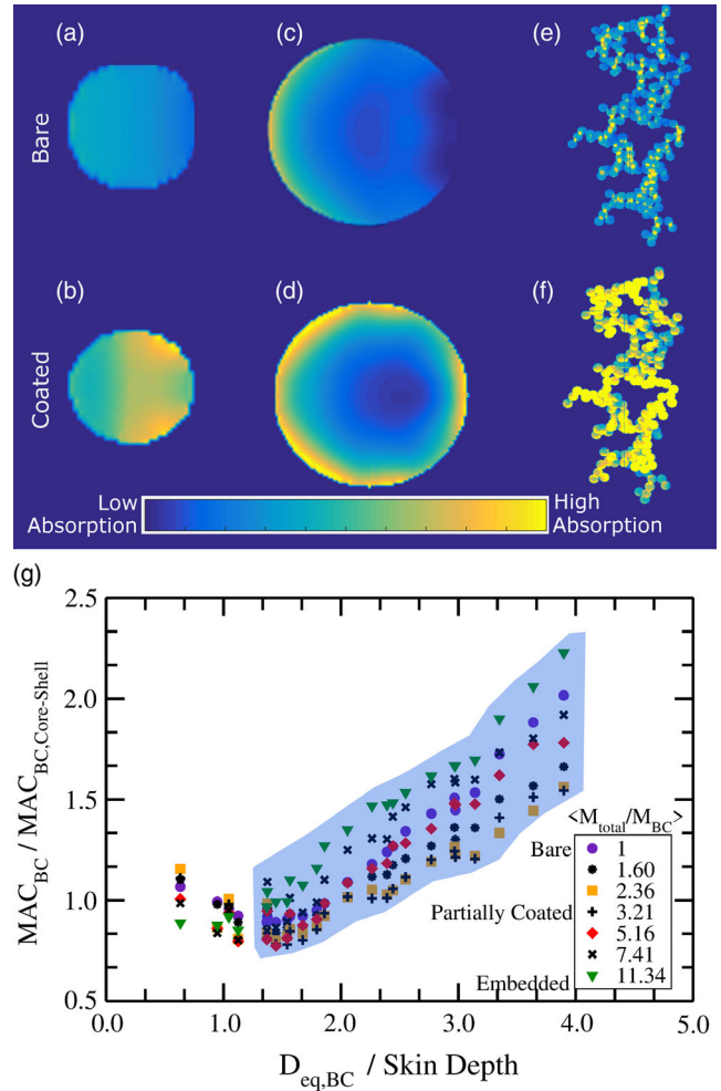
FIG. 4. Role of particle morphology in light absorption. The strength of internal light absorption is shown for BC particles in their bare and heavily coated states [panels (a)–(f)]. The coating material is nonabsorbing and is therefore invisible in this representation. The incident light impacts the particles from the left. (a) BC sphere of diameter of D = 80 nm; (b) same sphere as (a) but having a 90 nm thick layer of coating; (c) BC sphere of D = 300 nm; (d) same sphere as (c) but with a 260 nm coating; and (e) and (f) represent BC aggregates having volume equivalence to spheres in (c) and (d), respectively. Particles in (b), (d), and (f) are heavily coated which results in stronger absorption due to the lensing effect. The diameter of spherical BC cores in (c) and (d) is larger than the absorption skin depth resulting in the interior of the particle being excluded from contributing to light absorption. The BC aggregate is porous in structure and therefore light penetrates completely into it, allowing the entire volume to add to the total absorption [panels (e)–(f)]. (g) The \text{MAC}_{\text{BC}} ratios for coated aggregates to core shell is plotted versus the mass equivalent sphere diameter D_{\text{eq,BC}} divided by absorption skin depth. Significant disagreement is seen between the fractal and core-shell approximation models as D_{\text{eq,BC}} becomes greater than the skin depth. As the equivalent spheres become larger than the absorption skin depth, the core-shell model underpredicts the \text{MAC}_{\text{BC}} of the aggregates. The shaded region scales as (\text{MAC}_{\text{BC}}/\text{MAC}_{\text{BC,core-shell}}) \propto (D_{\text{eq,BC}}/\text{skin depth})^{0.75} .
