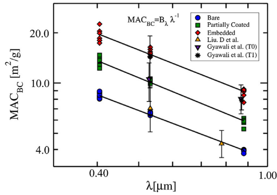
FIG. 3. Inverse wavelength scaling of BC mass absorption cross section ( \text{MAC}_{\text{BC}} ). The spectral response of MAC values for BC aggregates with varying degrees of mixing states are shown to follow an inverse functionality in wavelength (power law with exponent of -1 ). The fractal prefactor B_\lambda ranges from 3.5 (bare) to 5.2 (partially coated) to 7.8 (embedded), and denotes the enhancement in \text{MAC}_{\text{BC}} through the phenomenological “lensing effect.” Observational data sets collected over California, USA (Gyawali et al. [40]) and Manchester, UK (Liu et al. [13]) follow the scaling trends. Error bars indicate the standard deviation in the reported measurements.
