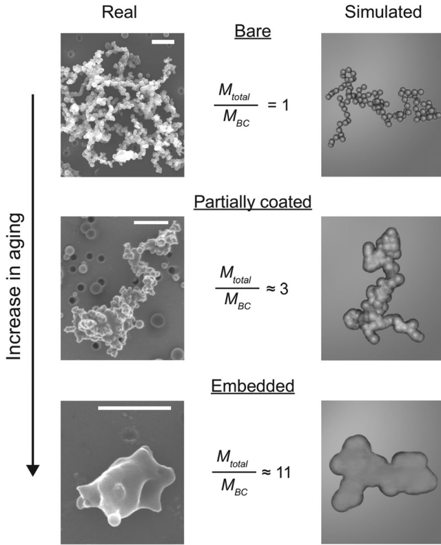
FIG. 1. Morphologies of internally mixed black carbon aggregates. Three simulated aggregates from this study that were “cherry picked” (shown in right column) demonstrate their close resemblance with real-world BC aerosol (left panel) corresponding to the three categories of internal mixing states as observed by China et al. [8]. The first-row particles represent bare BC aggregate with point contacting monomers and an open fractal morphology; partially coated aggregates are shown in the second row; and thickly coated or embedded aggregates are displayed in the third row. The total particle mass to BC mass ratio is shown in the center for each class of particle.
