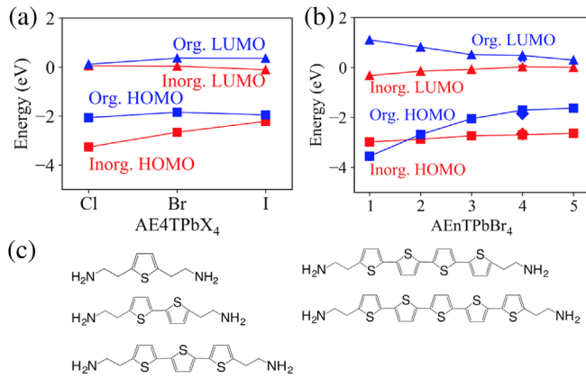
FIG. 3. (a) Frontier energy levels of the organic and inorganic components at the \Gamma point among the series of AE4TPbX 4 (X = Cl, Br, I). (b) Frontier energy levels at the \Gamma point among the series of AEnTPbBr 4 ( n = 1-5 ). Stars and diamonds indicate the energy levels of syn-anti-syn AE4TPbBr 4 for n = 4 . The average of Pb 1s energies is chosen to align the energy levels of different compounds. (c) Oligothiophene-based organic molecules considered in the all-anti configuration for varying the number n .
