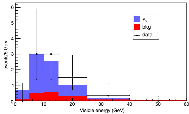
FIG. 1. Stacked plot of visible energy: data are compared with the expectation. Monte Carlo simulation is normalized to the expected number of events reported in Table 3.
