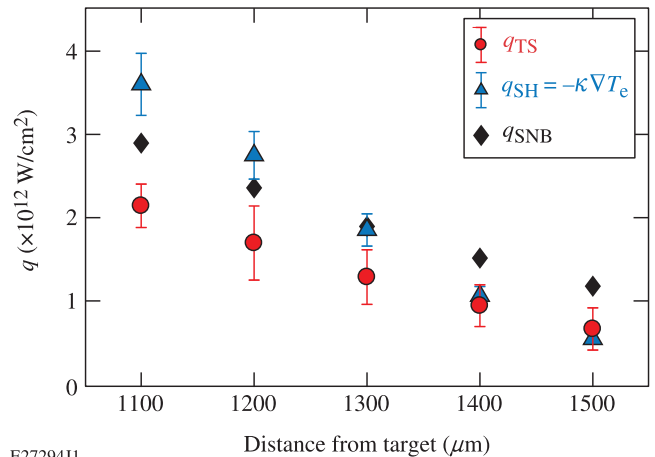
FIG. 3. The heat flux (red points) measured along the target normal is compared with classical heat flux (SH) calculations (blue points) and heat flux values (black points) obtained from the simulations using the SNB model. Both the simulations and calculations were initiated with the measured electron temperatures and densities. For reference, \lambda_{ei}/L_T = 1.4 \times 10^{-2} , 1.4 \times 10^{-2} , 1.3 \times 10^{-2} , 1.0 \times 10^{-2} , 7 \times 10^{-3} at 1.1, 1.2, 1.3, 1.4, and 1.5 mm, respectively.
