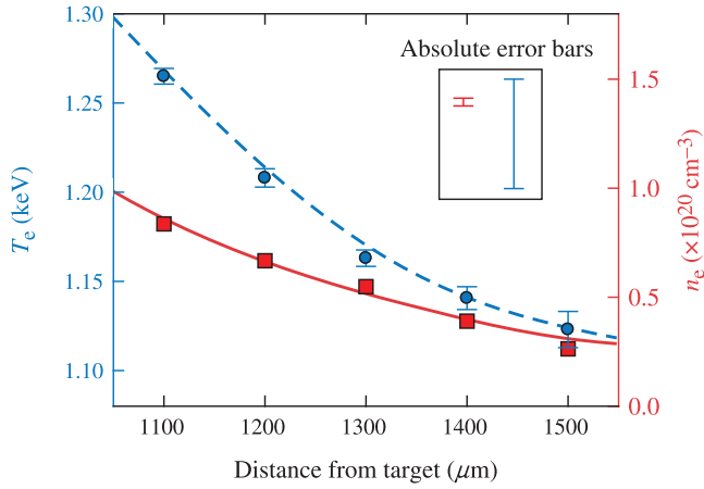
FIG. 4. Electron temperature (blue dots, left axis) and density (red squares, right axis) measurements at t = 1.5 ns. Profiles of electron temperature (dashed blue curve) and density (solid red curve) used in Fokker-Planck simulations. The relative ( 1\sigma statistical) error bars are shown with the temperature measurements. The absolute error bars are represented in the inset.
