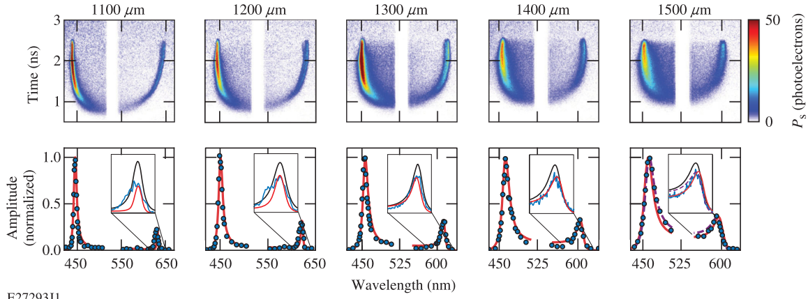
FIG. 2. The measured collective Thomson-scattering spectra (top row) and the corresponding spectral profiles (blue dots) at 1.5 ns (bottom row). The data were fit (red curves) with Eq. (1) using non-Maxwellian electron distribution functions to measure heat flux. Insets: The redshifted features are shown with calculations (black curves) that used the plasma conditions from the fit but a Maxwellian electron distribution function. These spectra recover the location of the scattering features but fail to match their amplitudes. At 1.5 mm, the spectrum was fit (dashed curve) with calculations that use a distribution function consistent with classical SH theory. All spectra are normalized to the peak scattered power.
