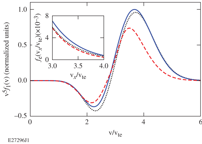
FIG. 5. The velocity-dependent contribution of heat flux is shown at 1200 \mu\text{m} for calculations using the Fokker-Planck (dashed red curve), classical (solid blue curve), and SNB (dotted black curve) models. Inset: The corresponding electron distribution functions are shown.
