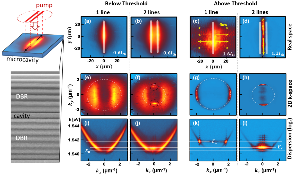
FIG. 1. (a)–(d) Real-space images of polariton emission when pumped with single or pairs of lines (as indicated in left schematic), both below and above the condensation threshold. (e)–(h) Corresponding momentum-space images of the entire polariton emission, white circles mark eventual condensation wave vector. (i)–(l) Cuts of the E(k) dispersion across the center of the dashed circles marked in (e)–(h).
