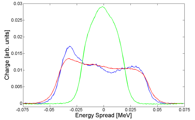
FIG. 5. Plots of three different 1D partial projections on energy. Each plot has a different number of fixed slits near the center of the beam. The green curve fixes two slits, the red curve fixes three, and the blue curve fixes four. The curves are normalized by area.
