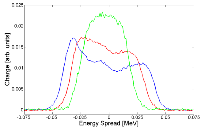
FIG. 6. Plots of partial projections on energy with three different beam currents. The green curve is from 20 mA, the red curve is from 30 mA, and the blue curve is from 40 mA. The correlation is more pronounced with increasing current, which indicates Coulomb forces cause the correlation. The curves are normalized by area.
