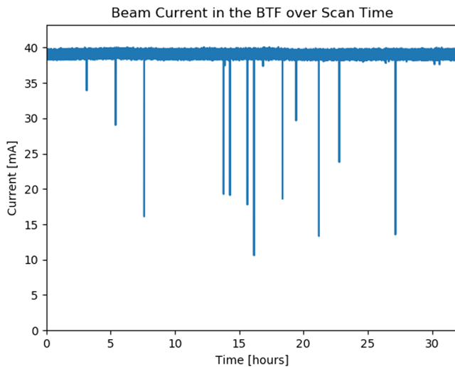
FIG. 2. The beam current upstream of the slits measured during the 6D scan.
