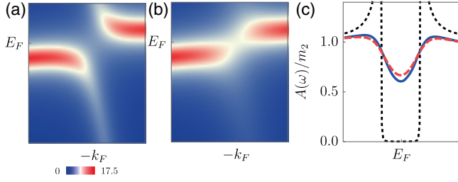
FIG. 2. (a) Spectral function A(k, \omega) for model \epsilon_i = k^2/(2m_i) - \mu_i ( i = 1, 2 ), m_2/m_1 = 50 , \delta(k_F)/(\mu_2 - \mu_1) = 0.02 , \Gamma_2/\delta(k_F) = 0.1 , \Gamma_1/\delta(k_F) = 0.7 , where the electron is spinless. The unit for the color bar is 1/\delta(k_F) . (b) Same as (a) but with \Gamma_1/\delta(k_F) = 1.7 . (c) Momentum-integrated spectral function A(\omega) for models in (a) (blue, solid) and (b) (red, dashed), and in the clean limit \Gamma_1 = \Gamma_2 = 0 (black, dotted). The unit for A(\omega) is m_2 .
