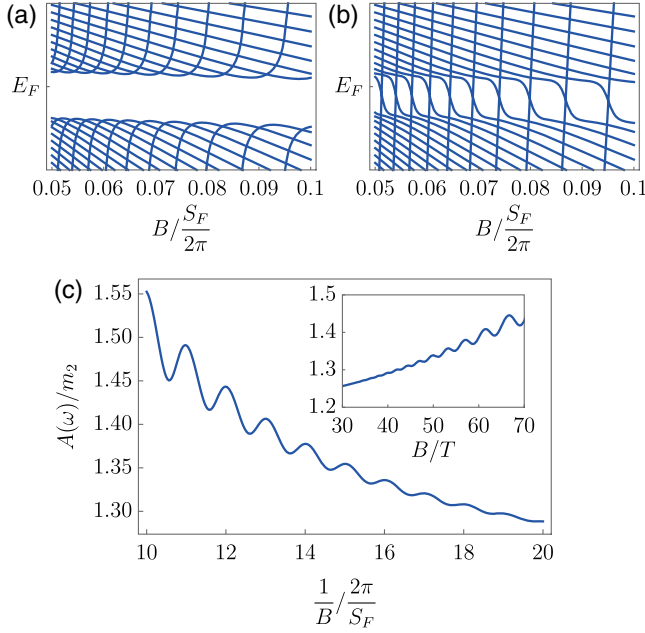
FIG. 3. (a) Real part of the Landau level spectrum \text{Re}[\mathcal{E}_{n,\pm}^\dagger] as a function of magnetic field, with the same model in Fig. 2(a). The s = \uparrow sector is similar. (b) Same as (a) but with the same model as Fig. 2(b). (c) Exact numerics of spectral function A(\omega = 0) as a function of 1/B and B (inset) with the model in (a). Here, both spin sectors are taken into account. The unit for A(\omega) is m_2 . m_1 = m_e is the free electron mass, and the hybridization gap is \delta(k_F) = 2 meV. The resulting indirect band gap is \delta = 0.56 meV, and the oscillation frequency is F = 800 T.
