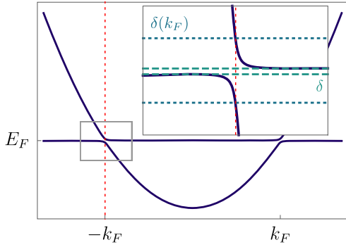
FIG. 1. Schematic band structure of a Kondo insulator. (Inset) Enlargement of the hybridization gap near k = k_F . \delta(k_F) is the hybridization gap defined as the energy difference of the two bands at k = k_F . \delta is the indirect band gap.
