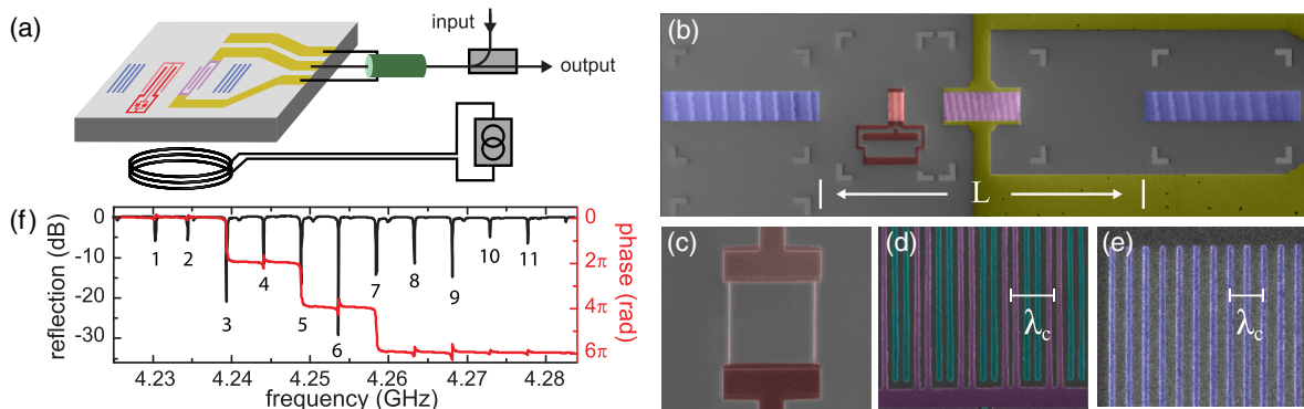
FIG. 1. Device diagram and acoustical cavity spectrum. (a) A cartoon schematic of the SAW cavity, acoustically coupled qubit, and the microwave network for control and measurement. (b) A false color SEM image of the fabricated device before the Josephson junction was patterned. Two Bragg reflectors (blue), each consisting of 400 Al strips, are spaced by L = 275 \mu\text{m} to define a SAW cavity, and a split-junction transmon qubit (red) was placed at L_{\text{eff}}/4 from the left reflector. A cavity-IDT (pink) with 125 periods at L/2 is used to drive and readout the cavity modes. The center and ground conductor of a coplanar waveguide (yellow) contact either side of the IDT. Measurements consist of detecting the reflection of a microwave tone applied to the cavity IDT. A directional coupler separates incident and reflected waves, so that the reflected signal is passed through a high electron mobility transistor (HEMT) amplifier and measured. False color SEM images of (c) a split Josephson junction with a 7 \times 7 \mu\text{m}^2 loop area, (d) a split-finger IDT with the upper electrode in green and the lower in purple [29], and (e) several Al stripes within a Bragg reflector. The characteristic wavelength of the cavity is indicated, \lambda_c = v_s/f_c = 677 nm, where the center frequency is f_c = 4.253 GHz. (f) A microwave reflection measurement of the SAW cavity reveals 11 (numbered) prominent longitudinal modes within the mirror bandwidth.
