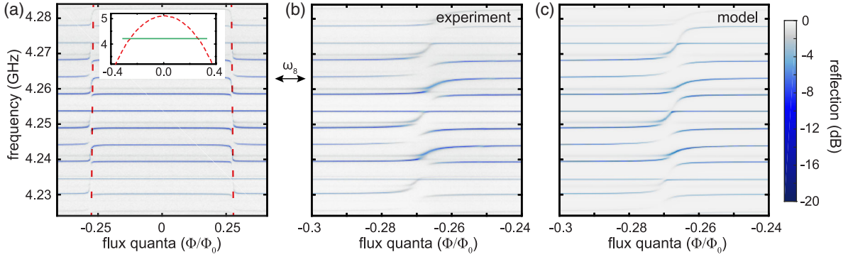
FIG. 2. Resonantly coupled multimode CQAD system. (a) The plot shows the cavity reflection (color scale) as the transmon is tuned by varying the applied magnetic flux. The red dashed line indicates the transmon’s flux dependent resonance. The inset shows the expected qubit frequency (red), which has a maximum at 5.08 GHz. The green section indicates the measured range of panel (a). (b) Enlargement of the first set of avoided crossings shown in panel (a). (c) A model for the acoustic spectrum based on the interaction Hamiltonian, Eq. (2).
