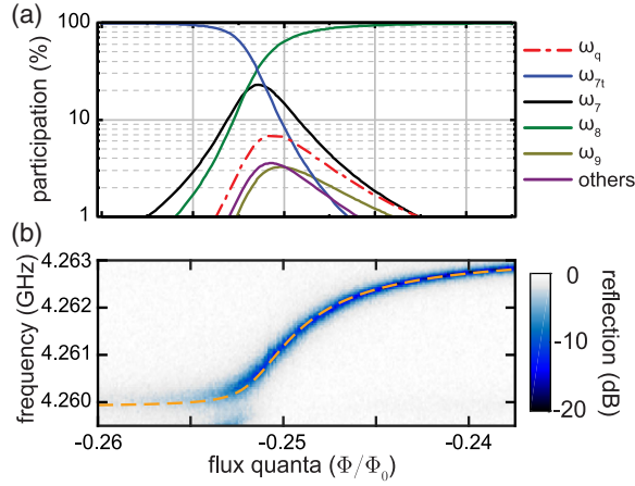
FIG. 3. Hybridization of modes in the strong multimode regime. (a) The solid lines show the squared coefficients of the eigenvector (participation) in the uncoupled mode basis as the qubit tunes with magnetic field. At -0.252 flux quanta, longitudinal modes \omega_7 and \omega_8 and transverse mode \omega_{7t} nearly equally contribute to 89% of the eigenvector. The “others” trace shows the combined contribution of the remaining modes. (b) The acoustic spectrum [from Fig. 2(b)] between modes \omega_7 and \omega_8 . The dotted line shows the eigenvalue fit from the model corresponding to the superposition of modes from (a).
