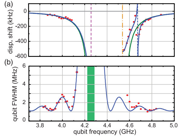
FIG. 4. Measurements in the dispersive regime. (a) The dispersive shift of cavity mode \omega_8 versus qubit frequency ( \omega_q ). The purple, orange, and blue dashed lines indicate \omega_8/2\pi , \omega_8/2\pi + \alpha , and \omega_8/2\pi + 3\alpha/2 , respectively, where \alpha = 273 MHz is the transmon’s anharmonicity [29]. The green line shows a prediction from the standard transmon model, and the solid blue line shows a prediction from diagonalizing a generalized Jaynes-Cummings Hamiltonian with a 4-level transmon. (b) The qubit linewidth versus qubit frequency. Red points are measurements, and the blue line shows the expected spontaneous emission rate of the qubit into SAWs based on the qubit-IDT geometry, with an offset to account for the intrinsic decoherence, i.e., processes other than spontaneous emission that decohere the qubit. The green region indicates the mirror bandwidth.
