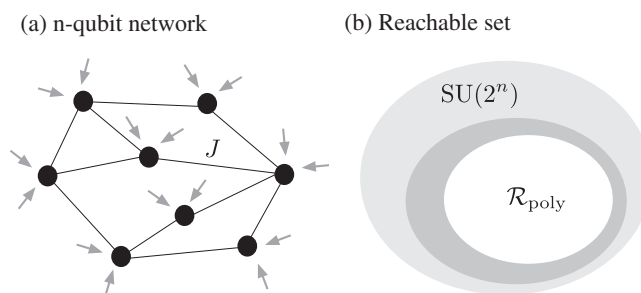
FIG. 1. Illustration of one of the main results: (a) for a generic qubit network (3) in which each qubit is subject to two local controls (4) (gray arrows), (b) the set of gates \mathcal{R}_{\text{poly}} (white area) that (provably) can be implemented in a time that scales at most polynomially in the number of qubits is characterized [see Eq. (2)]. The dark gray area represents the set of gates that can be reached with time optimal methods in polynomial time.
