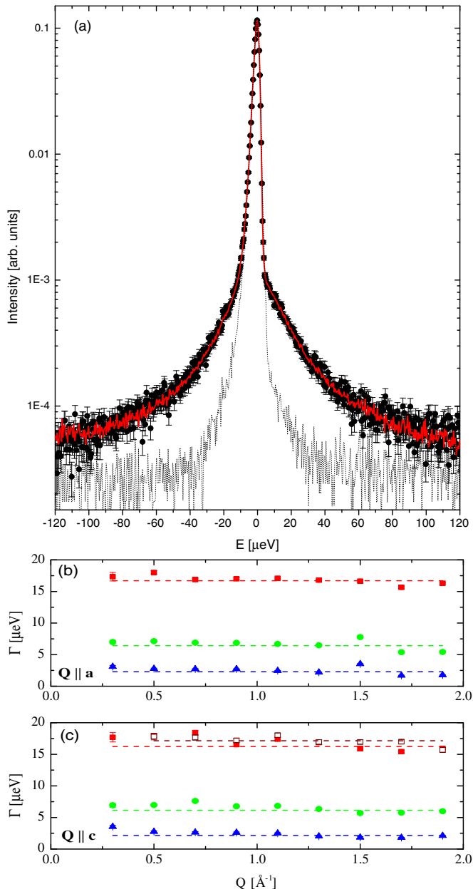
FIG. 2. Panel (a) illustrates BASIS measurements of the dynamic structure factor S(\mathbf{Q}, E) of hemimorphite at T = 100 K when \mathbf{Q} \parallel c and Q = 1.50 \text{ \AA}^{-1} . The intrinsic half-width at half-maximum \Gamma of the Lorentzian component observed at BASIS is shown in panels (b) and (c). Solid symbols in both panels show the observed widths when Q = 0.70 \text{ \AA}^{-1} is exactly parallel to the specified crystal direction. The blue, green, and red symbols correspond to 80, 90, and 100 K, respectively. Open symbols in (c) plot the intrinsic widths \Gamma when Q = 1.50 \text{ \AA}^{-1} is exactly parallel to c . Error bars throughout the text represent one standard deviation.
