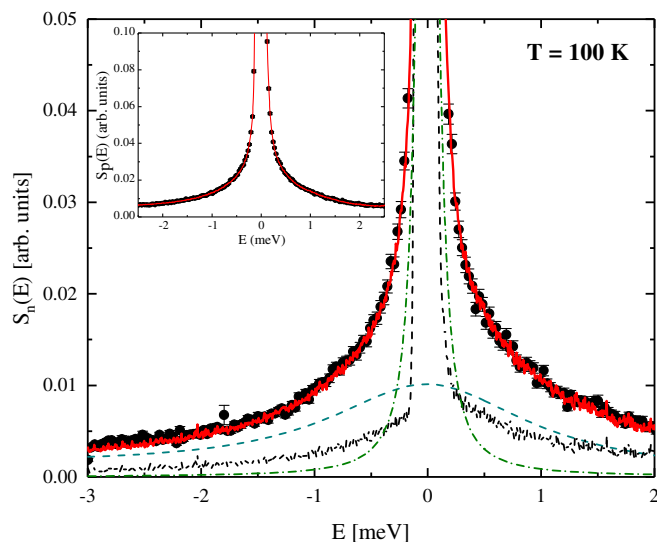
FIG. 3. The observed inelastic scattering function S(E) obtained via CNCS. A fit to the scattering data from the negative-angle detectors with the following symbol designations: Experimental data (black circles), broad Lorentzian component plus linear background (dashed dark cyan line), narrow Lorentzian component (dash-dotted green line), elastic scattering (dotted black line), and total fit function (solid red curve). The insert plots the data from the positive-angle detectors.
