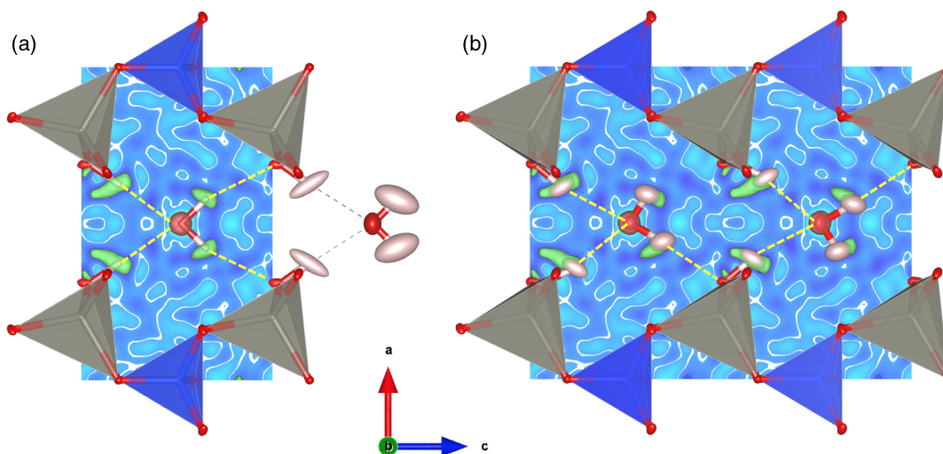
FIG. 1. The crystal structure of hemimorphite viewed along the b axis. The framework is shown as a traditional ball-and-stick model with anisotropic displacement parameters at 65% probability. The hydroxyl proton and the water molecule are shown as nuclear density isosurfaces. Panel (a) illustrates model A for phase I, and panel (b) illustrates the unit cell for phase II. Model B for phase I is the same as shown on panel (b) with random occupancy of the water molecules. Figure designations: Nuclear density isosurfaces for water oxygens (red), nuclear density isosurfaces for water or hydroxyl protons (green), SiO_4 tetrahedra (blue), ZnO_3(OH) tetrahedra (gray), framework oxygen (red).
