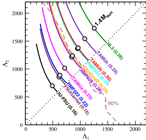
FIG. 2. Tidal polarizabilities \Lambda_1 and \Lambda_2 associated with the high-mass M_1 and low-mass M_2 components of the binary predicted by a set of ten distinct RMF models. Models to the right side of the 90% probability contour extracted from Ref. [2] are ruled out. The solid circles represent model predictions for a BNS system having masses of M_1 = 1.4 M_{\odot} and M_2 = 1.33 M_{\odot} , respectively.
