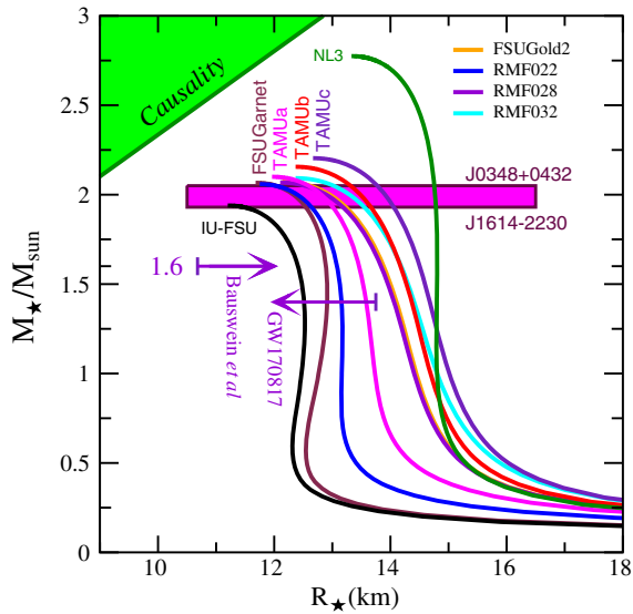
FIG. 4. Mass-vs-radius relation predicted by the ten RMF models discussed in the text. Mass constraints obtained from electromagnetic observations of two neutron stars are indicated with a combined uncertainty bar [45,46]. In contrast, the arrows indicate constraints on stellar radii obtained exclusively from GW170817 and exclude many of the otherwise acceptable EOSs. The excluded causality region was adopted from Fig. 2 of Ref. [55].
