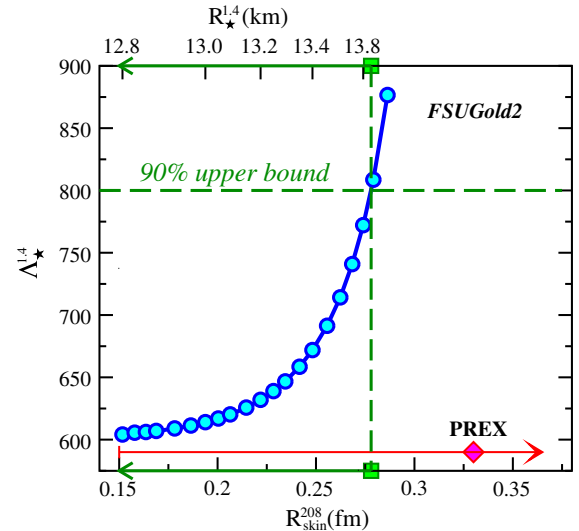
FIG. 1. The dimensionless tidal polarizability \Lambda_{\star}^{1.4} of a 1.4M_{\odot} neutron star as a function of the neutron-skin thickness of ^{208}\text{Pb} (lower abscissa) and the radius of a 1.4M_{\odot} neutron star (upper abscissa) as predicted by the FSUGold2 family of relativistic interactions. Constraints on R_{\text{skin}}^{208} and R_{\star}^{1.4} are inferred from adopting the \Lambda_{\star}^{1.4} \leq 800 limit deduced from GW170817 [2].
