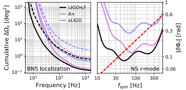
FIG. 5. Left: The cumulative uncertainty in localization, \Delta\Omega_s , for the HLI network. We consider NS binaries at the Coma cluster with two inclinations, 30^\circ (solid line) and 75^\circ (dashed line), and marginalize over the polarization and time of arrival. LIGO-LF improves the localization by a factor of 3.5 over aLIGO using the entire signal and by a factor of 5 over A+ using only the sub-30 Hz data. Right: The uncertainty (solid line) in measuring the phase shift due to the resonant excitation of the NS r mode \delta\Phi_r as a function of the NS spin frequency f_{\text{spin}} . We consider the single detector case and fix the sources at 50 Mpc with optimal orientation. Also shown in the red dashed line is the expected physical r -mode phase shift. The effect is detectable when the real phase shift is greater than the statistical error.
