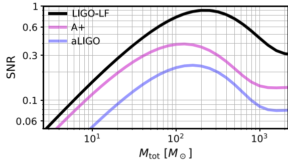
FIG. 6. SNR from the GW memory effect as a function of the source-frame total mass. The sources are fixed at z = 0.1 and an inclination of 30^\circ . The peak SNR seen in LIGO-LF is 4 (2) times greater than that seen in aLIGO (A+).
