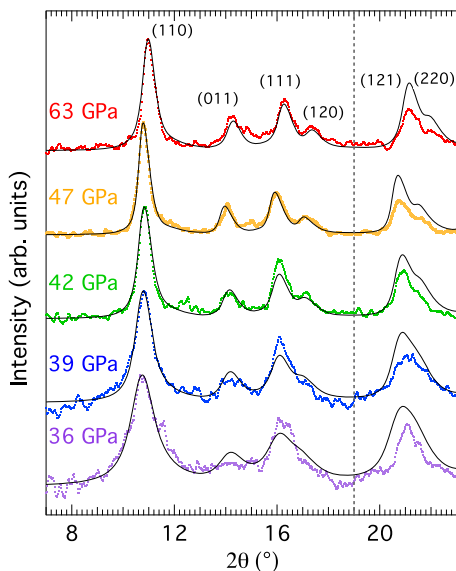
FIG. 2. X-ray diffraction data in the high-pressure region. The fits (black curves) overlay experimental data (points). Least-squares fits were performed to determine the lattice parameters and peak widths for stishovite diffraction peaks. The vertical dotted line denotes the extent of the fit region, above which detector-sensitivity effects render intensity data quantitatively unreliable.
