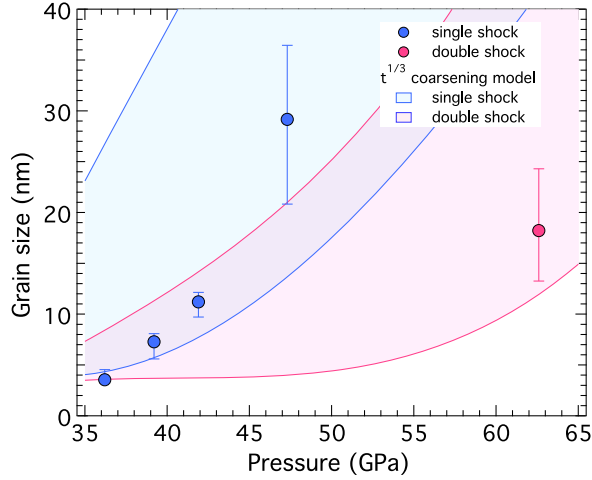
FIG. 4. Grain sizes determined using the Scherrer equation from the current experiments (circles) along with range of grain sizes predicted using the t^{1/3} coarsening law from molecular dynamics [53] for both single-shock (blue field) and double-shock (pink field) states. The large uncertainties in grain size calculations arise primarily from uncertainty in the shock temperature.
