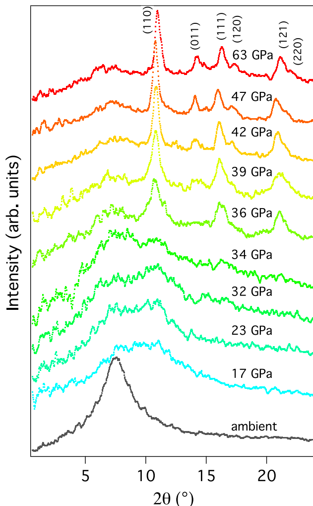
FIG. 1. Azimuthally integrated x-ray diffraction data collected for a series of plate-impact experiments with peak stress states between 17 and 63 GPa. Stishovite peaks are labeled with hkl values.
