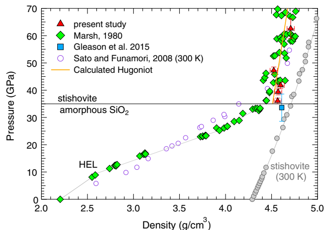
FIG. 3. Shock Hugoniot curve for fused silica. Red triangles show x-ray densities from this study. Continuum Hugoniot data from gun experiments [50] are shown as green diamonds along with the x-ray density (blue square) determined from laser-driven compression [25]. Also shown are 300-K static compression data for stishovite (gray circles) [51] and fused silica (open purple circles) [52]. HEL (Hugoniot elastic limit).
